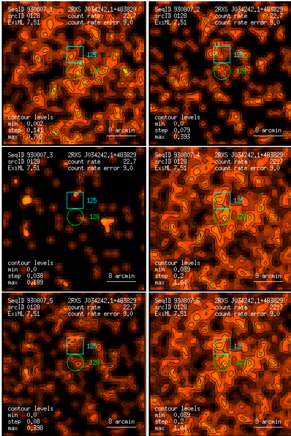
Figure 128: RASS 930807: detection 0128: band rate images, Gaussian filter: (1) PSPC channels 11 – 41, (2) 52 – 90, (3) 91 – 201, (4) 11 – 235, (5) 52 – 201, (6) 11 – 201. Broad band rates in counts/ks. Band rate contour levels in counts/ks/arcmin 2 .
