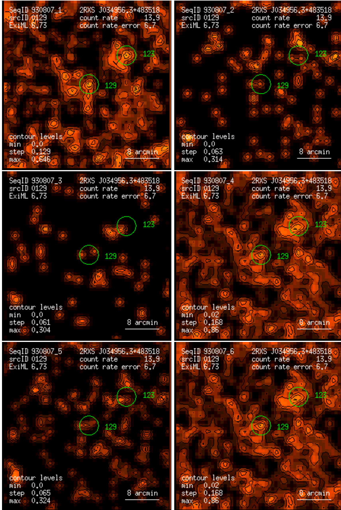
Figure 129: RASS 930807: detection 0129: band rate images, Gaussian filter: (1) PSPC channels 11 – 41, (2) 52 – 90, (3) 91 – 201, (4) 11 – 235, (5) 52 – 201, (6) 11 – 201. Broad band rates in counts/ks. Band rate contour levels in counts/ks/arcmin 2 .
