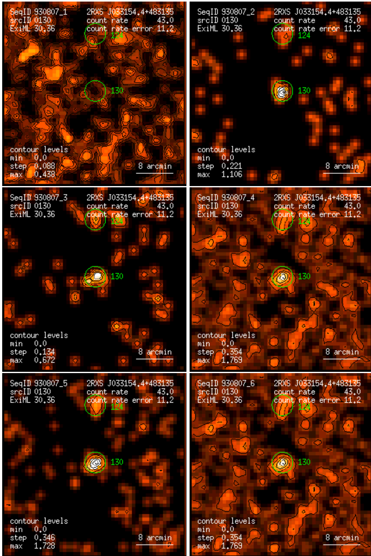
Figure 130: RASS 930807: detection 0130: band rate images, Gaussian filter: (1) PSPC channels 11 – 41, (2) 52 – 90, (3) 91 – 201, (4) 11 – 235, (5) 52 – 201, (6) 11 – 201. Broad band rates in counts/ks. Band rate contour levels in counts/ks/arcmin 2 .
