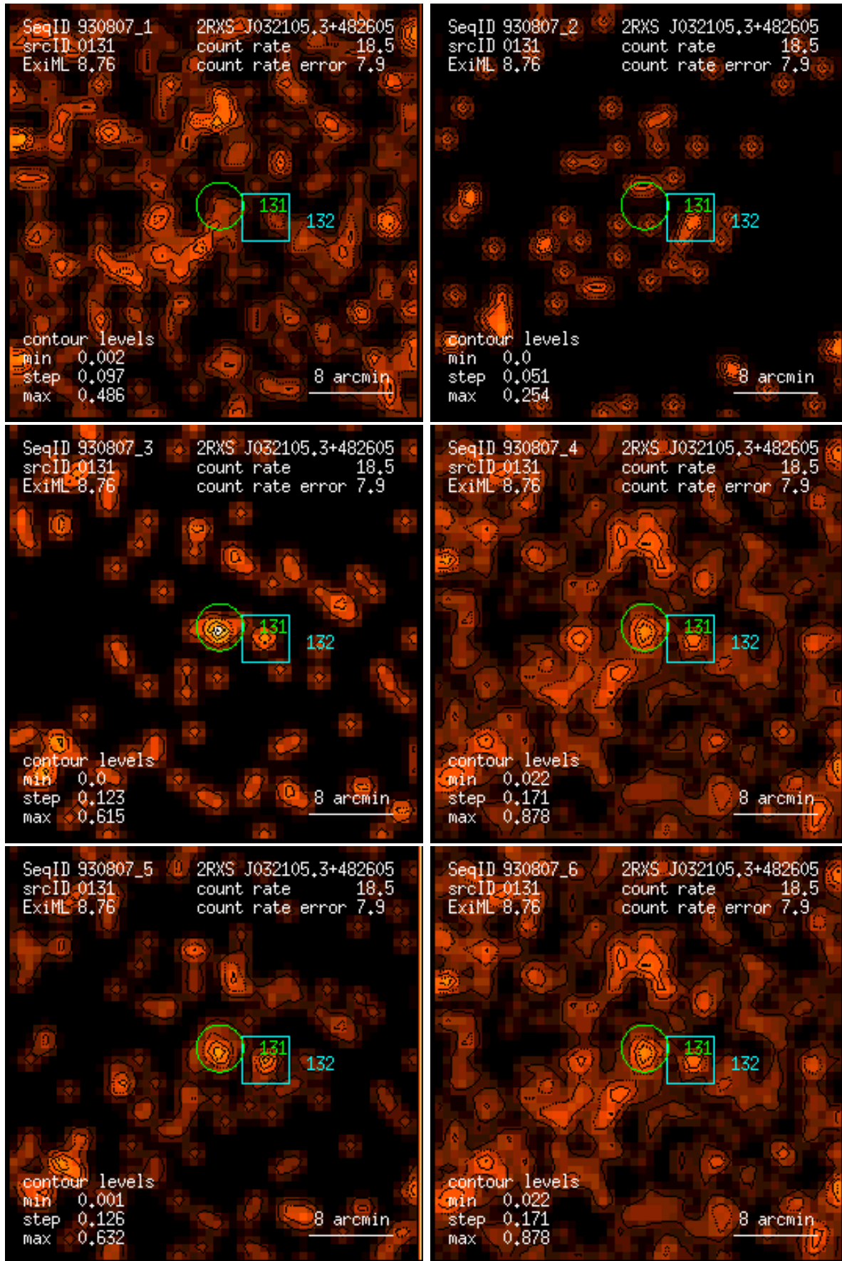
Figure 131: RASS 930807: detection 0131: band rate images, Gaussian filter: (1) PSPC channels 11 – 41, (2) 52 – 90, (3) 91 – 201, (4) 11 – 235, (5) 52 – 201, (6) 11 – 201. Broad band rates in counts/ks. Band rate contour levels in counts/ks/arcmin 2 .
