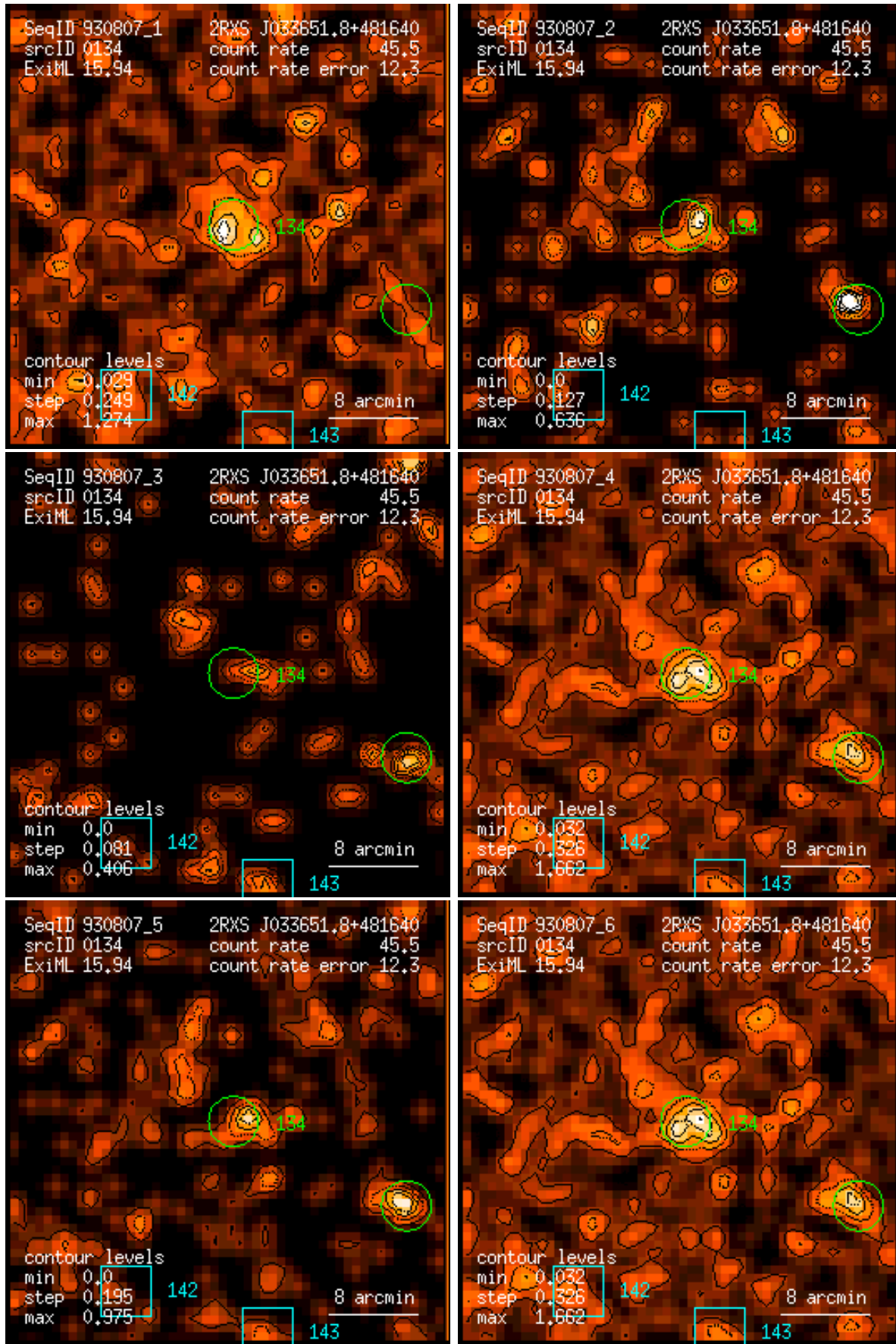
Figure 134: RASS 930807: detection 0134: band rate images, Gaussian filter: (1) PSPC channels 11 – 41, (2) 52 – 90, (3) 91 – 201, (4) 11 – 235, (5) 52 – 201, (6) 11 – 201. Broad band rates in counts/ks. Band rate contour levels in counts/ks/arcmin 2 .
