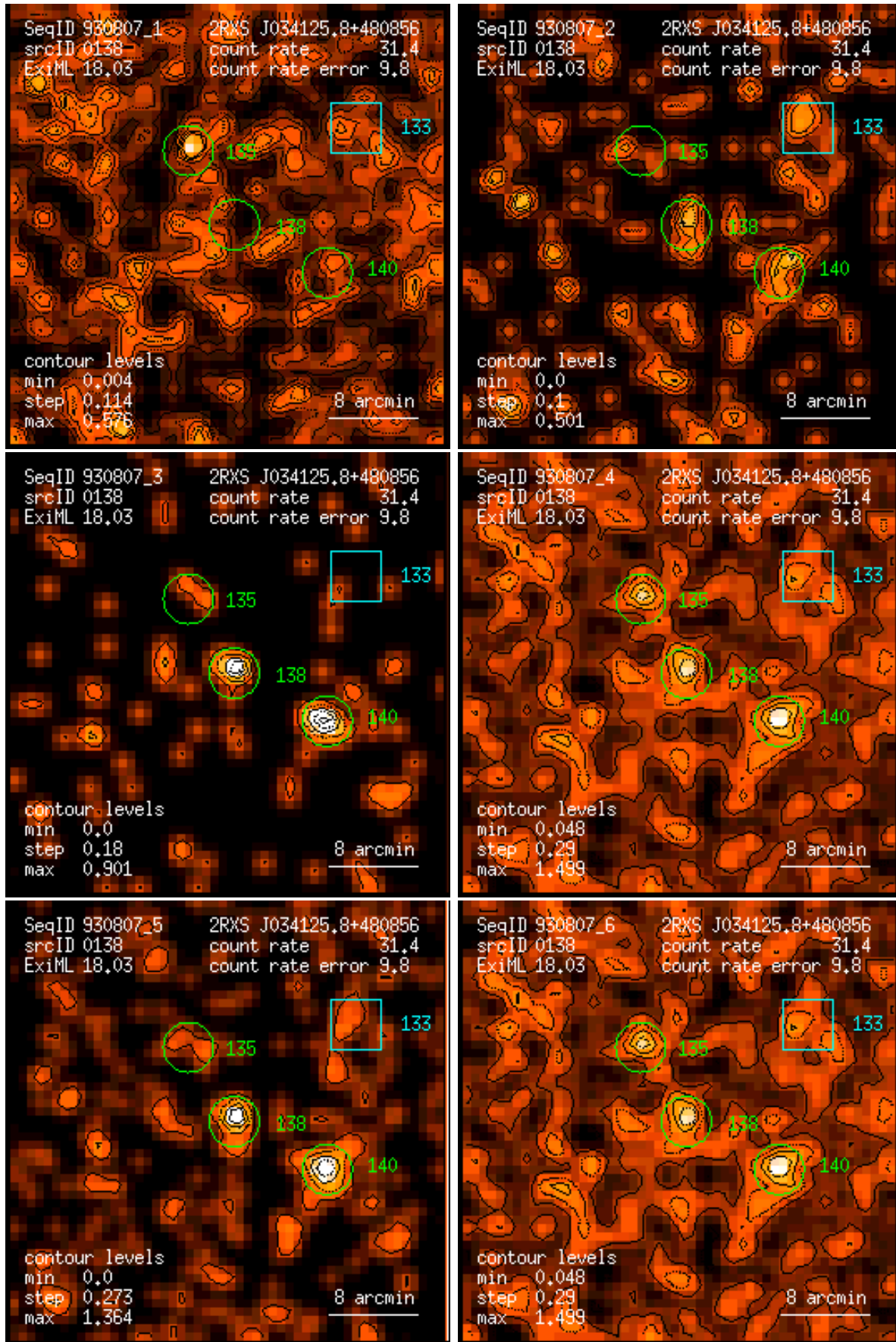
Figure 138: RASS 930807: detection 0138: band rate images, Gaussian filter: (1) PSPC channels 11 – 41, (2) 52 – 90, (3) 91 – 201, (4) 11 – 235, (5) 52 – 201, (6) 11 – 201. Broad band rates in counts/ks. Band rate contour levels in counts/ks/arcmin 2 .
