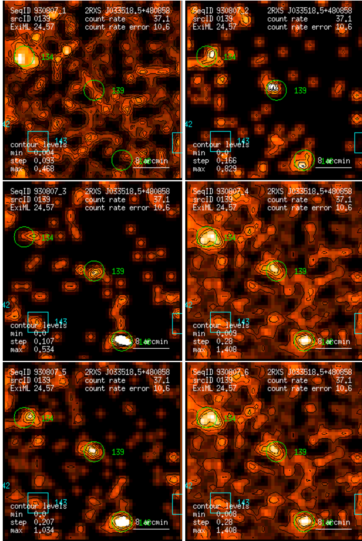
Figure 139: RASS 930807: detection 0139: band rate images, Gaussian filter: (1) PSPC channels 11 – 41, (2) 52 – 90, (3) 91 – 201, (4) 11 – 235, (5) 52 – 201, (6) 11 – 201. Broad band rates in counts/ks. Band rate contour levels in counts/ks/arcmin 2 .
