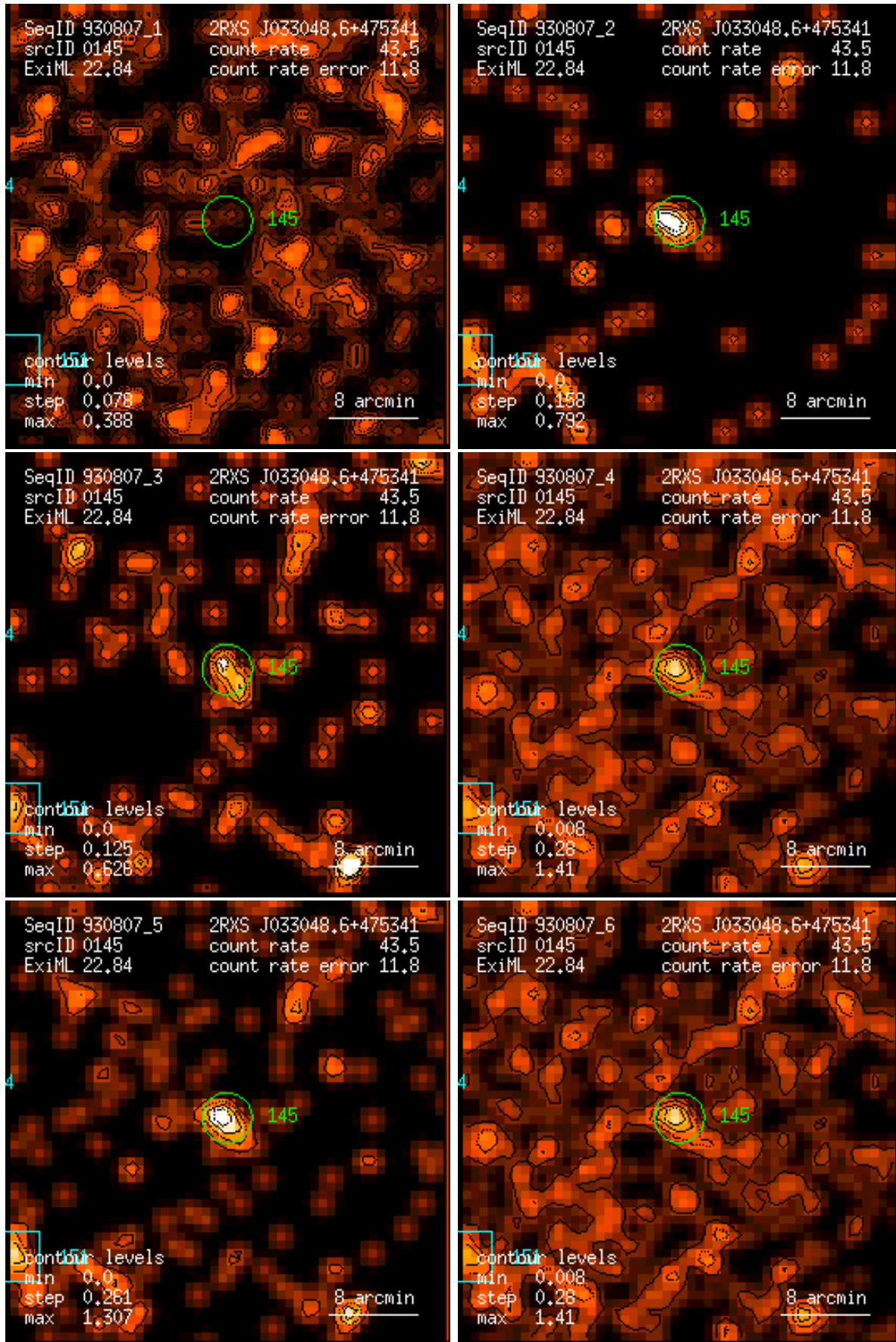
Figure 145: RASS 930807: detection 0145: band rate images, Gaussian filter: (1) PSPC channels 11 – 41, (2) 52 – 90, (3) 91 – 201, (4) 11 – 235, (5) 52 – 201, (6) 11 – 201. Broad band rates in counts/ks. Band rate contour levels in counts/ks/arcmin 2 .
