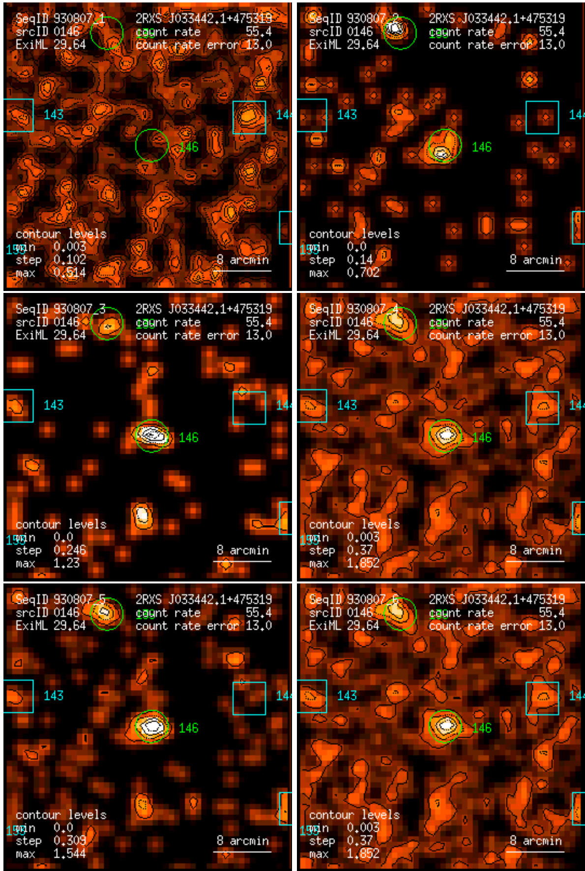
Figure 146: RASS 930807: detection 0146: band rate images, Gaussian filter: (1) PSPC channels 11 – 41, (2) 52 – 90, (3) 91 – 201, (4) 11 – 235, (5) 52 – 201, (6) 11 – 201. Broad band rates in counts/ks. Band rate contour levels in counts/ks/arcmin 2 .
