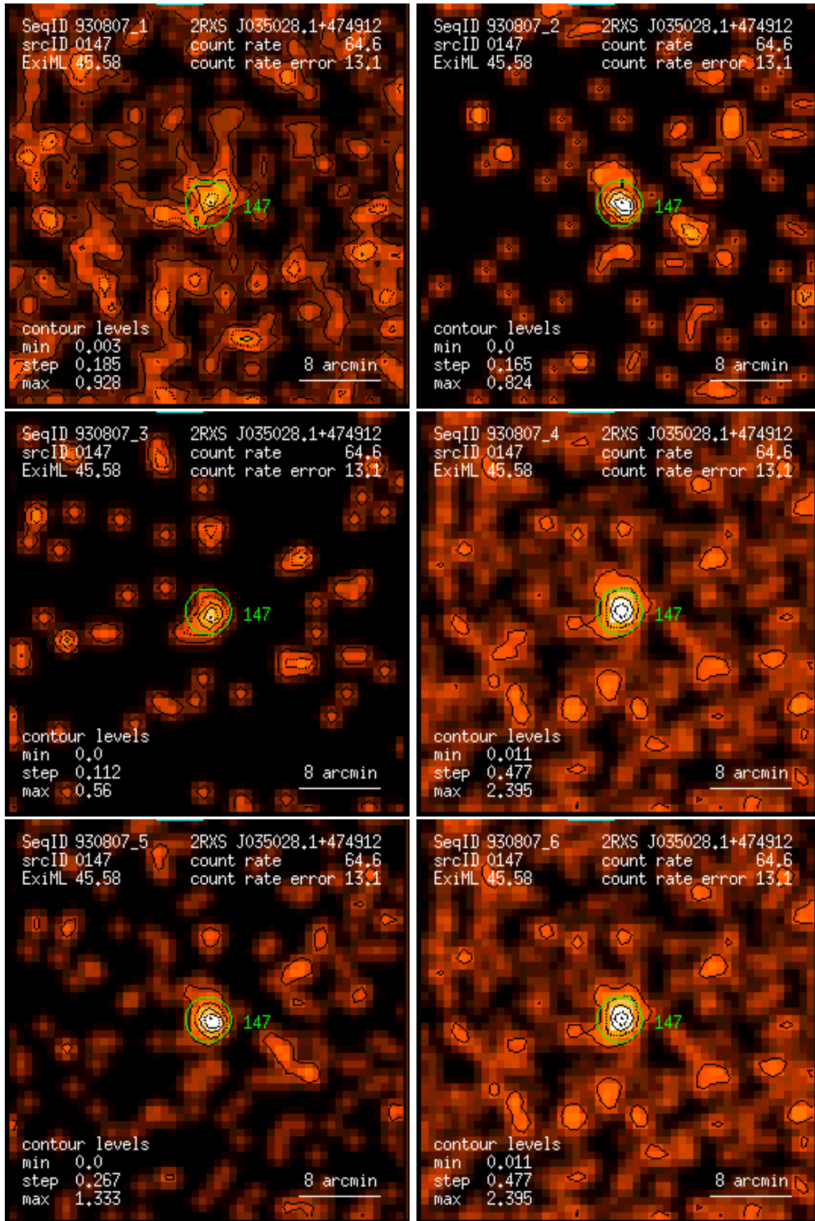
Figure 147: RASS 930807: detection 0147: band rate images, Gaussian filter: (1) PSPC channels 11 – 41, (2) 52 – 90, (3) 91 – 201, (4) 11 – 235, (5) 52 – 201, (6) 11 – 201. Broad band rates in counts/ks. Band rate contour levels in counts/ks/arcmin 2 .
