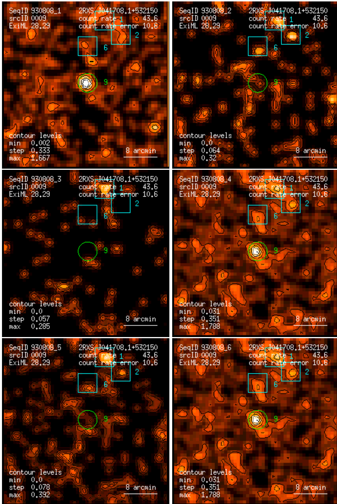
Figure 9: RASS 930808: detection 0009: band rate images, Gaussian filter: (1) PSPC channels 11 – 41, (2) 52 – 90, (3) 91 – 201, (4) 11 – 235, (5) 52 – 201, (6) 11 – 201. Broad band rates in counts/ks. Band rate contour levels in counts/ks/arcmin 2 .
