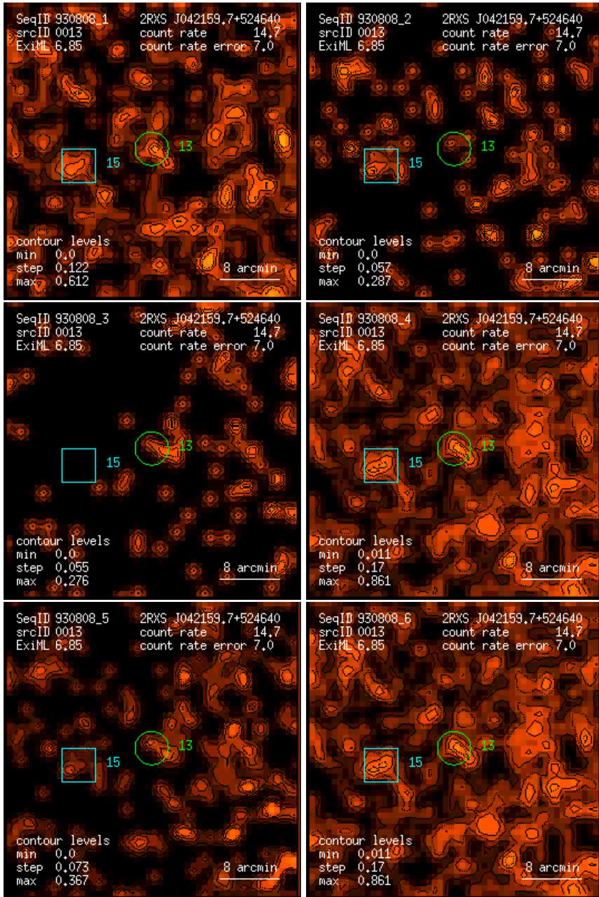
Figure 13: RASS 930808: detection 0013: band rate images, Gaussian filter: (1) PSPC channels 11 – 41, (2) 52 – 90, (3) 91 – 201, (4) 11 – 235, (5) 52 – 201, (6) 11 – 201. Broad band rates in counts/ks. Band rate contour levels in counts/ks/arcmin 2 .
