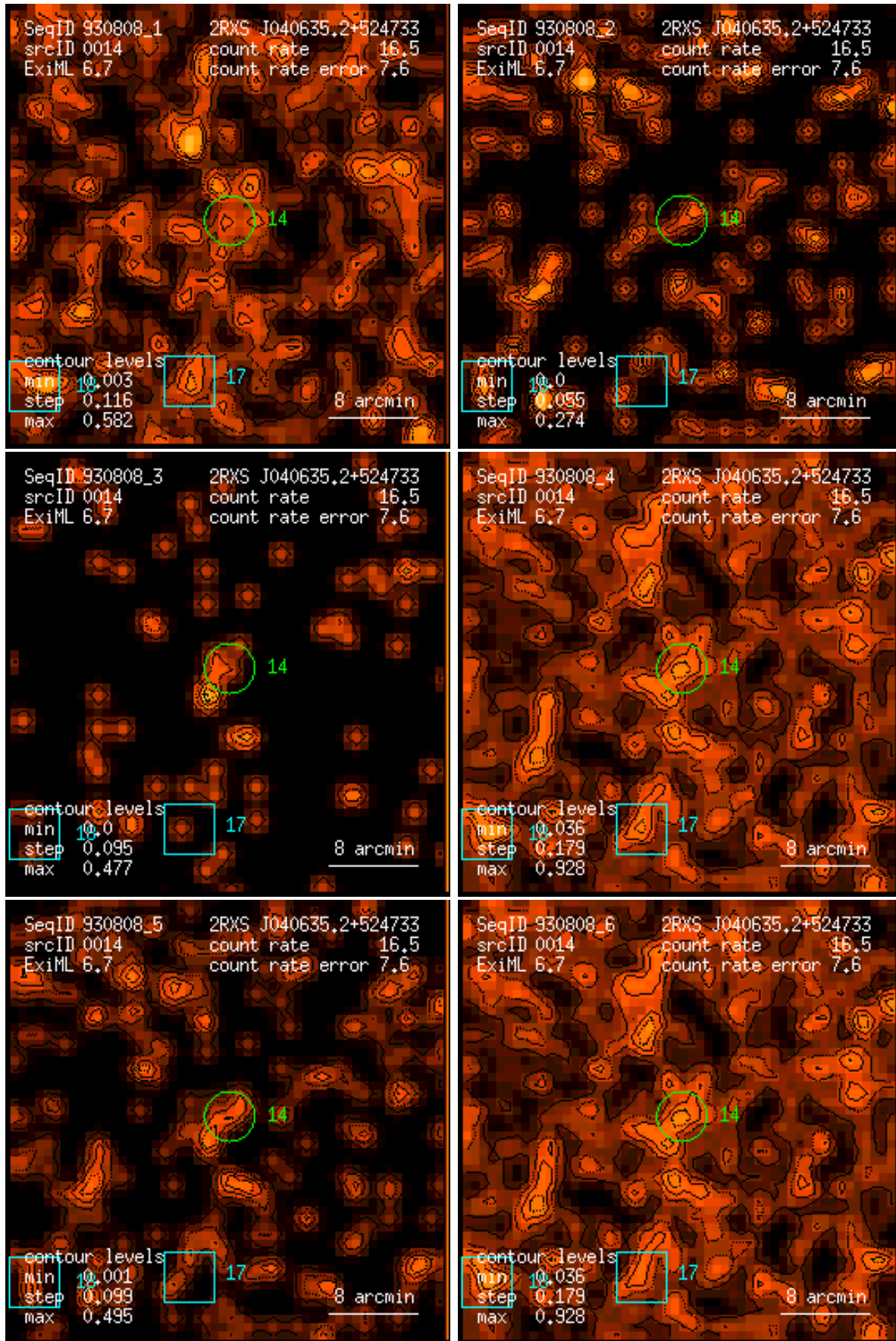
Figure 14: RASS 930808: detection 0014: band rate images, Gaussian filter: (1) PSPC channels 11 – 41, (2) 52 – 90, (3) 91 – 201, (4) 11 – 235, (5) 52 – 201, (6) 11 – 201. Broad band rates in counts/ks. Band rate contour levels in counts/ks/arcmin 2 .
