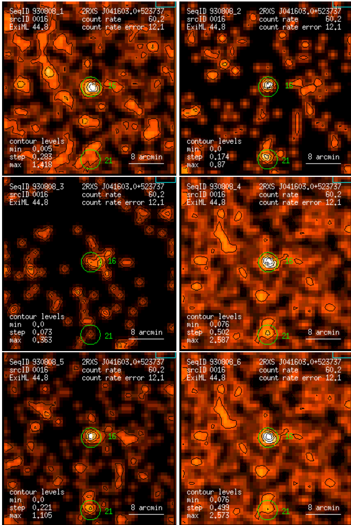
Figure 16: RASS 930808: detection 0016: band rate images, Gaussian filter: (1) PSPC channels 11 – 41, (2) 52 – 90, (3) 91 – 201, (4) 11 – 235, (5) 52 – 201, (6) 11 – 201. Broad band rates in counts/ks. Band rate contour levels in counts/ks/arcmin 2 .
