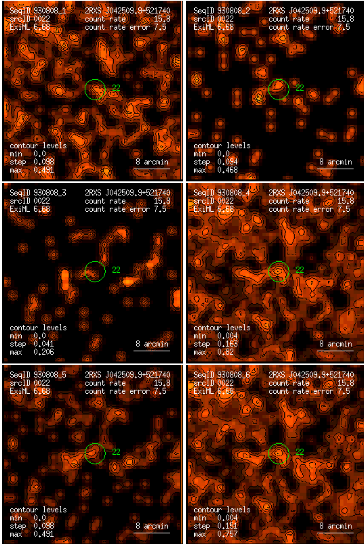
Figure 22: RASS 930808: detection 0022: band rate images, Gaussian filter: (1) PSPC channels 11 – 41, (2) 52 – 90, (3) 91 – 201, (4) 11 – 235, (5) 52 – 201, (6) 11 – 201. Broad band rates in counts/ks. Band rate contour levels in counts/ks/arcmin 2 .
