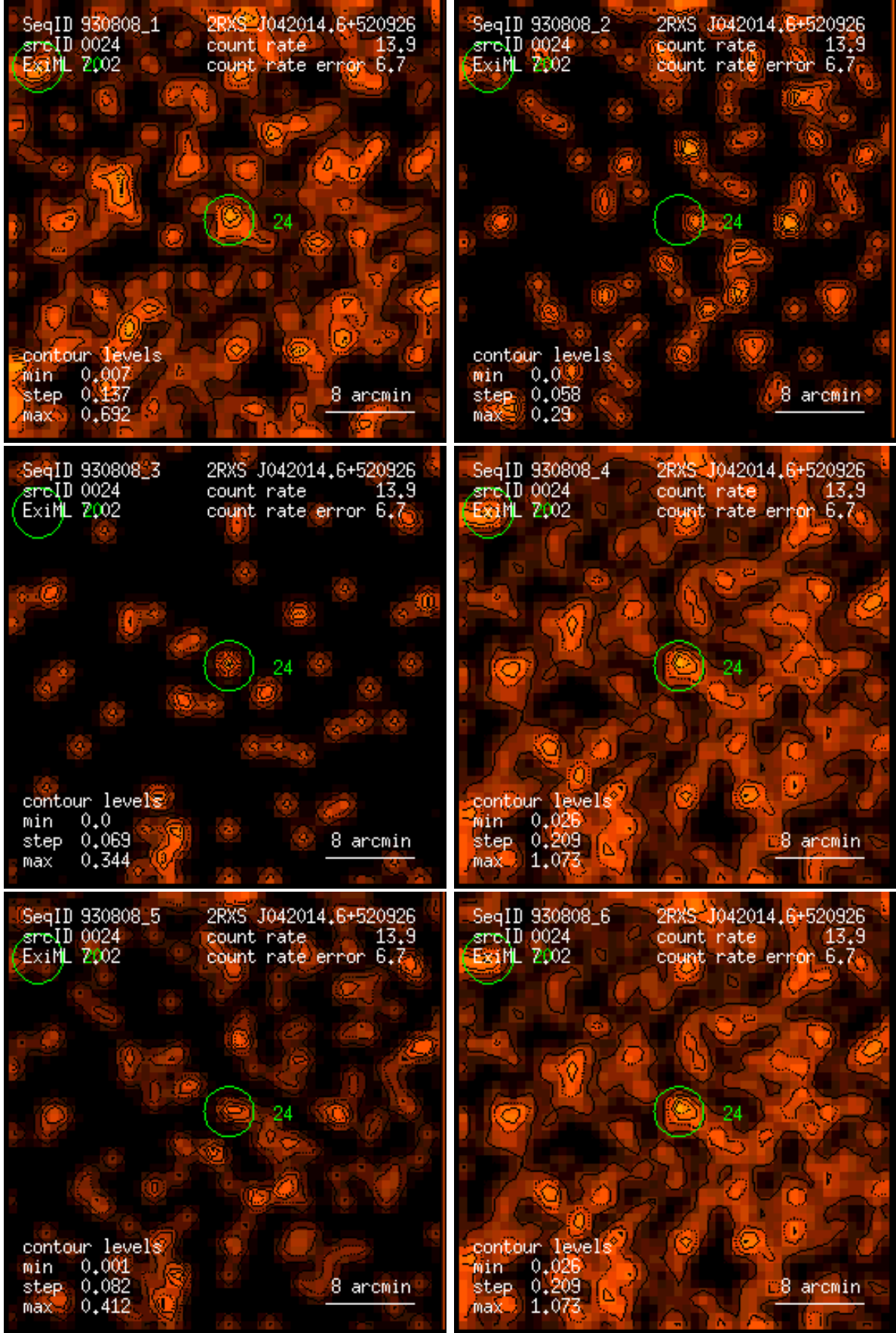
Figure 24: RASS 930808: detection 0024: band rate images, Gaussian filter: (1) PSPC channels 11 – 41, (2) 52 – 90, (3) 91 – 201, (4) 11 – 235, (5) 52 – 201, (6) 11 – 201. Broad band rates in counts/ks. Band rate contour levels in counts/ks/arcmin 2 .
