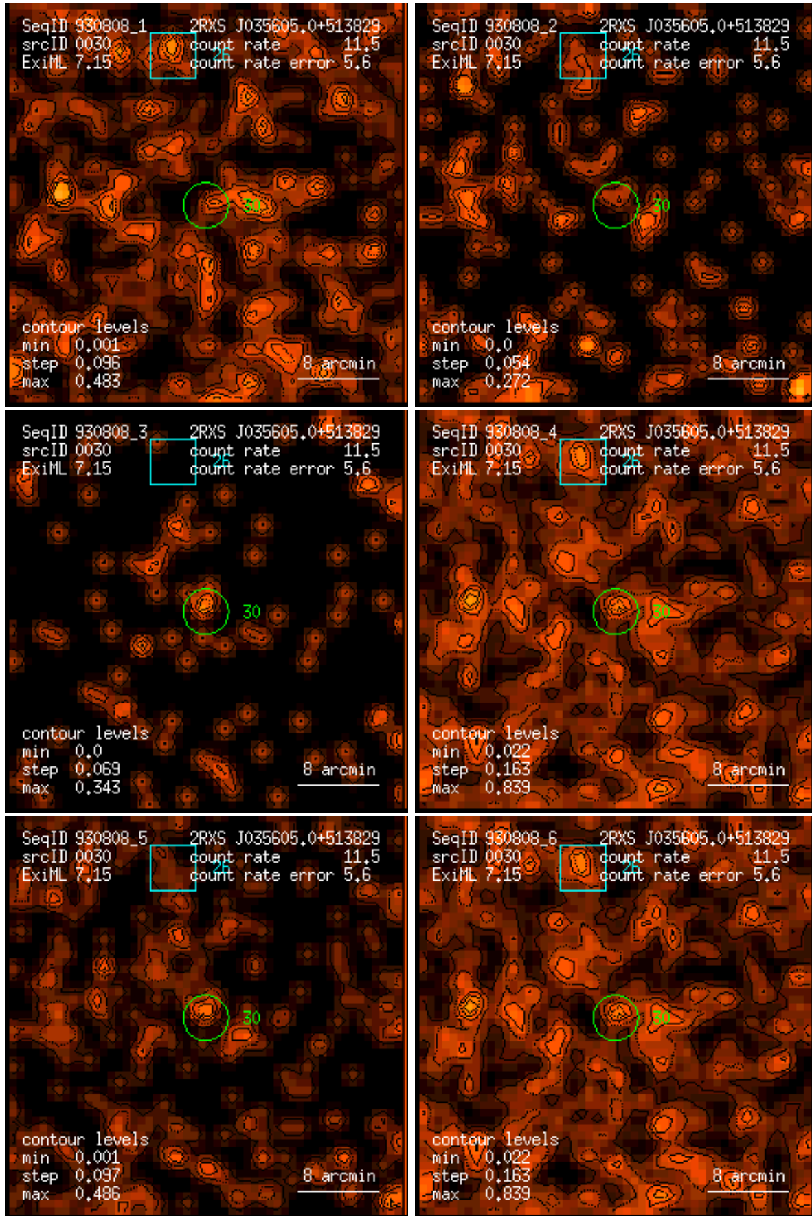
Figure 30: RASS 930808: detection 0030: band rate images, Gaussian filter: (1) PSPC channels 11 – 41, (2) 52 – 90, (3) 91 – 201, (4) 11 – 235, (5) 52 – 201, (6) 11 – 201. Broad band rates in counts/ks. Band rate contour levels in counts/ks/arcmin 2 .
