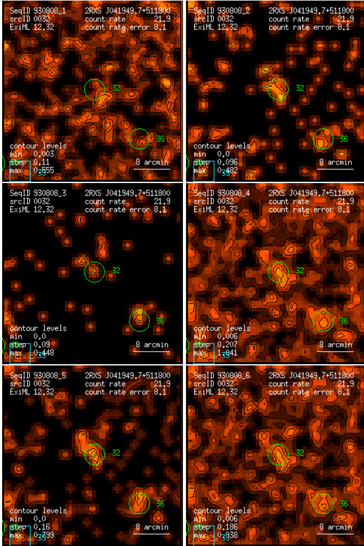
Figure 32: RASS 930808: detection 0032: band rate images, Gaussian filter: (1) PSPC channels 11 – 41, (2) 52 – 90, (3) 91 – 201, (4) 11 – 235, (5) 52 – 201, (6) 11 – 201. Broad band rates in counts/ks. Band rate contour levels in counts/ks/arcmin 2 .
