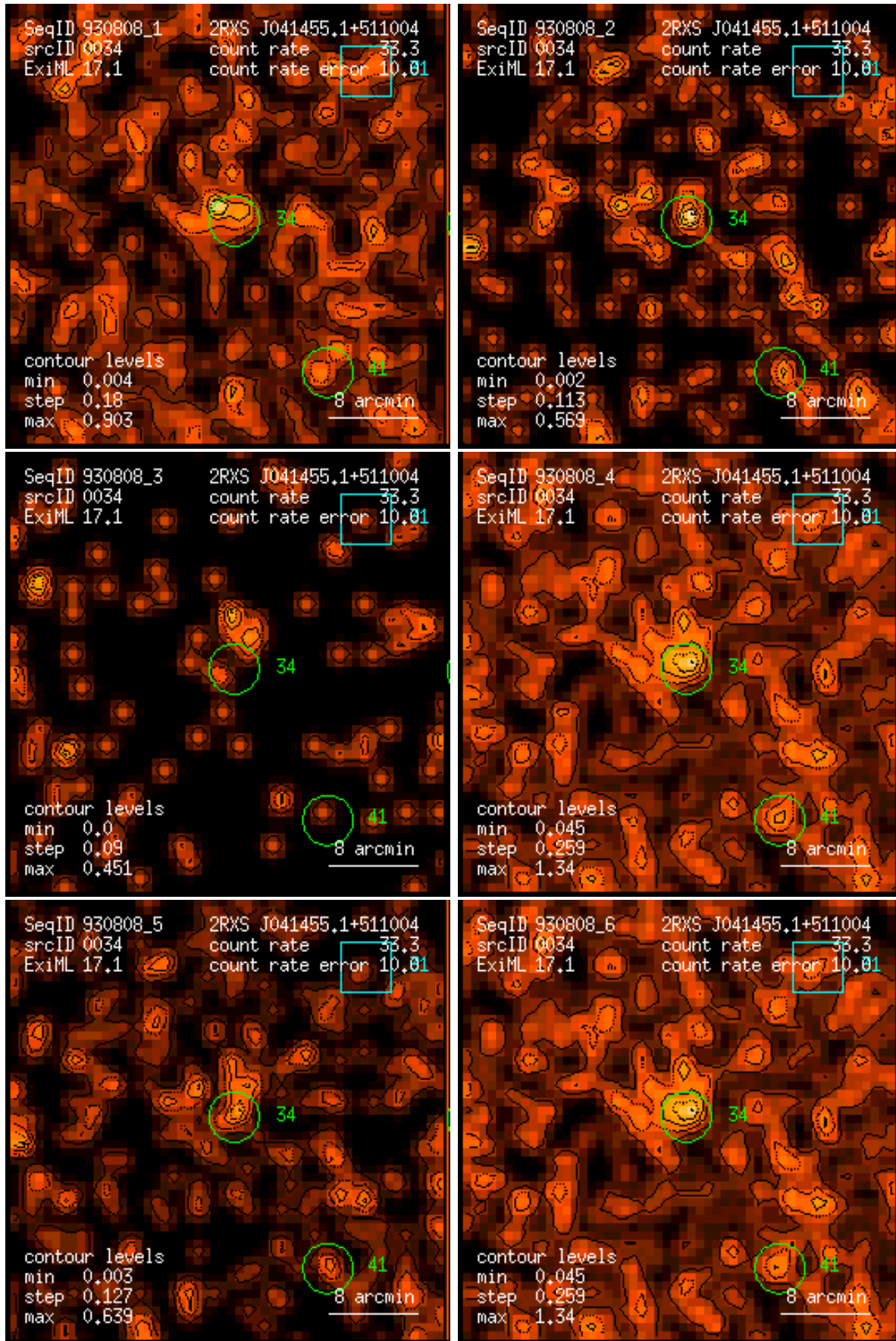
Figure 34: RASS 930808: detection 0034: band rate images, Gaussian filter: (1) PSPC channels 11 – 41, (2) 52 – 90, (3) 91 – 201, (4) 11 – 235, (5) 52 – 201, (6) 11 – 201. Broad band rates in counts/ks. Band rate contour levels in counts/ks/arcmin 2 .
