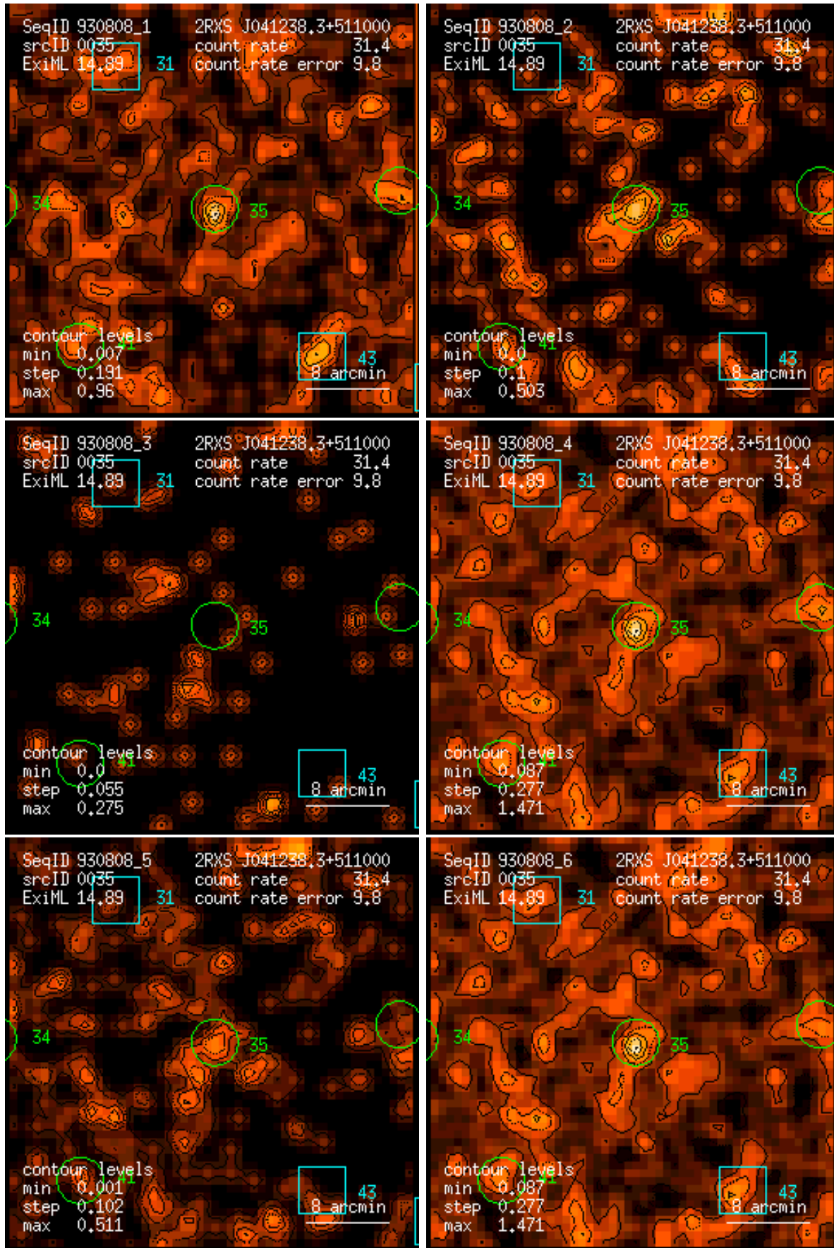
Figure 35: RASS 930808: detection 0035: band rate images, Gaussian filter: (1) PSPC channels 11 – 41, (2) 52 – 90, (3) 91 – 201, (4) 11 – 235, (5) 52 – 201, (6) 11 – 201. Broad band rates in counts/ks. Band rate contour levels in counts/ks/arcmin 2 .
