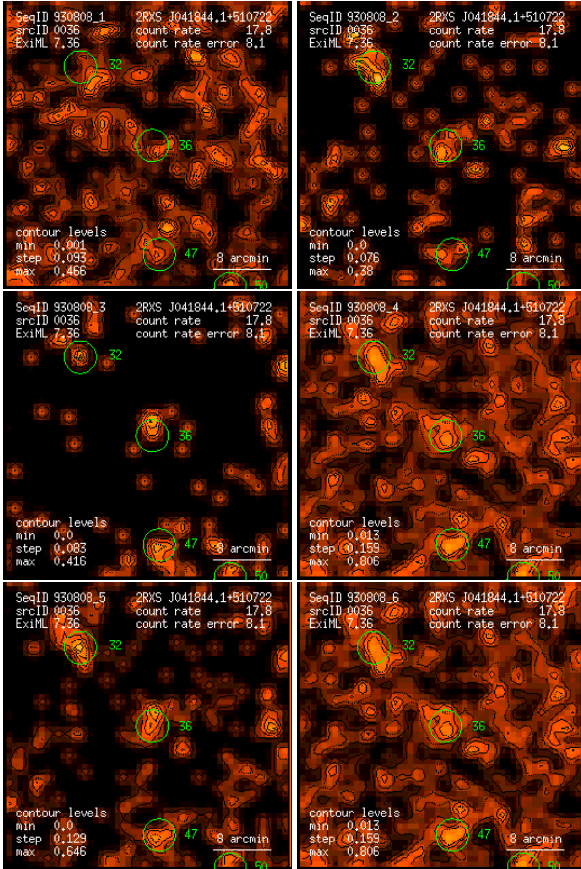
Figure 36: RASS 930808: detection 0036: band rate images, Gaussian filter: (1) PSPC channels 11 – 41, (2) 52 – 90, (3) 91 – 201, (4) 11 – 235, (5) 52 – 201, (6) 11 – 201. Broad band rates in counts/ks. Band rate contour levels in counts/ks/arcmin 2 .
