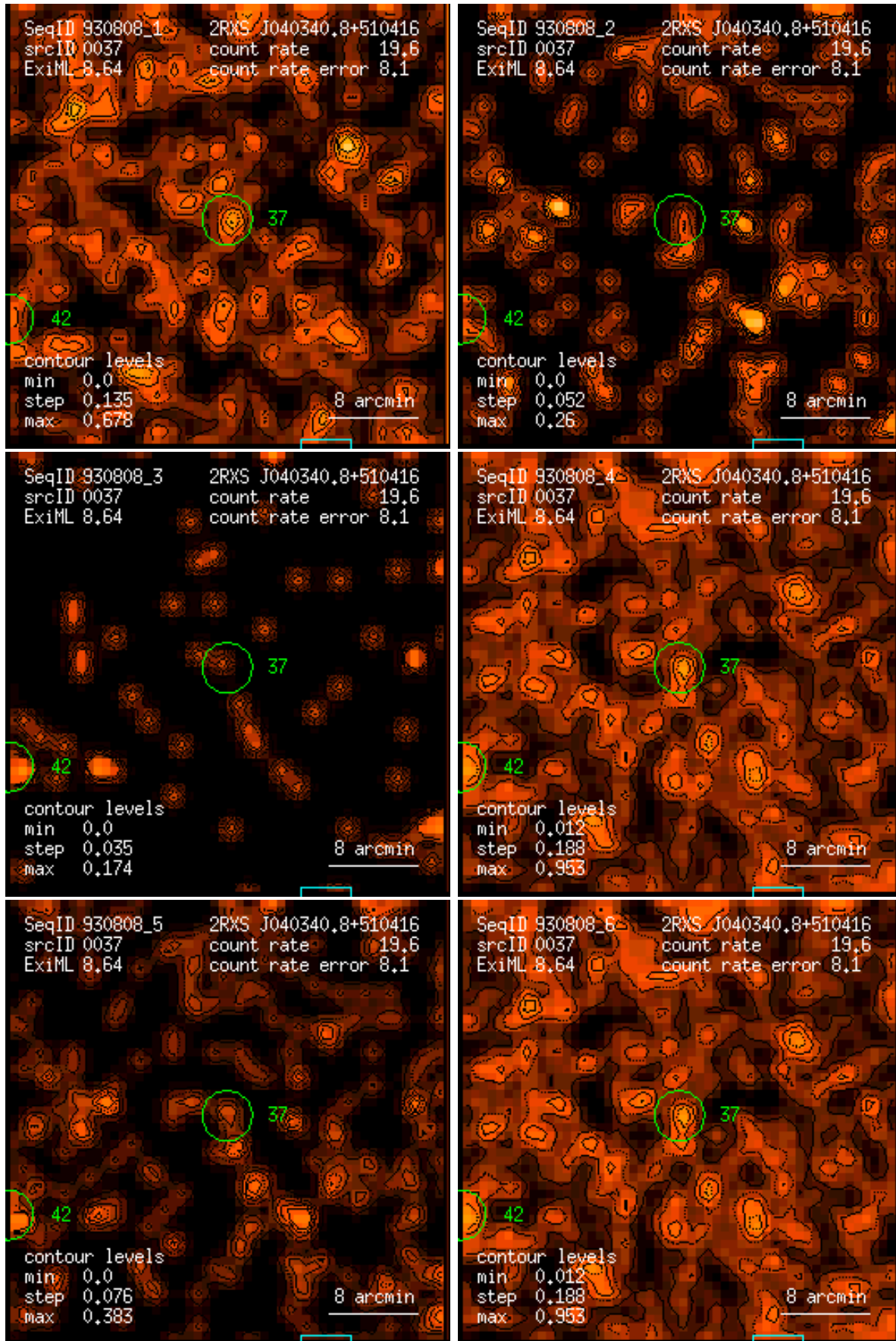
Figure 37: RASS 930808: detection 0037: band rate images, Gaussian filter: (1) PSPC channels 11 – 41, (2) 52 – 90, (3) 91 – 201, (4) 11 – 235, (5) 52 – 201, (6) 11 – 201. Broad band rates in counts/ks. Band rate contour levels in counts/ks/arcmin 2 .
