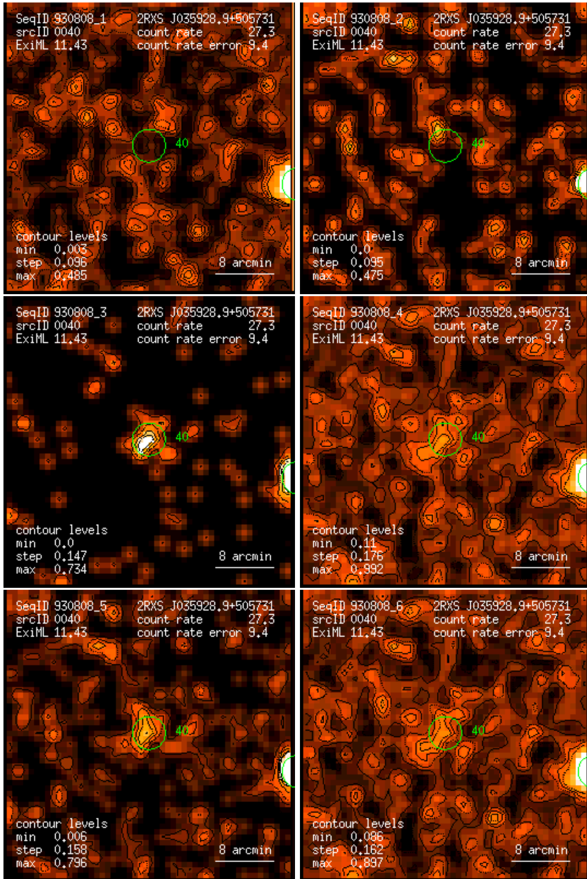
Figure 40: RASS 930808: detection 0040: band rate images, Gaussian filter: (1) PSPC channels 11 – 41, (2) 52 – 90, (3) 91 – 201, (4) 11 – 235, (5) 52 – 201, (6) 11 – 201. Broad band rates in counts/ks. Band rate contour levels in counts/ks/arcmin 2 .
