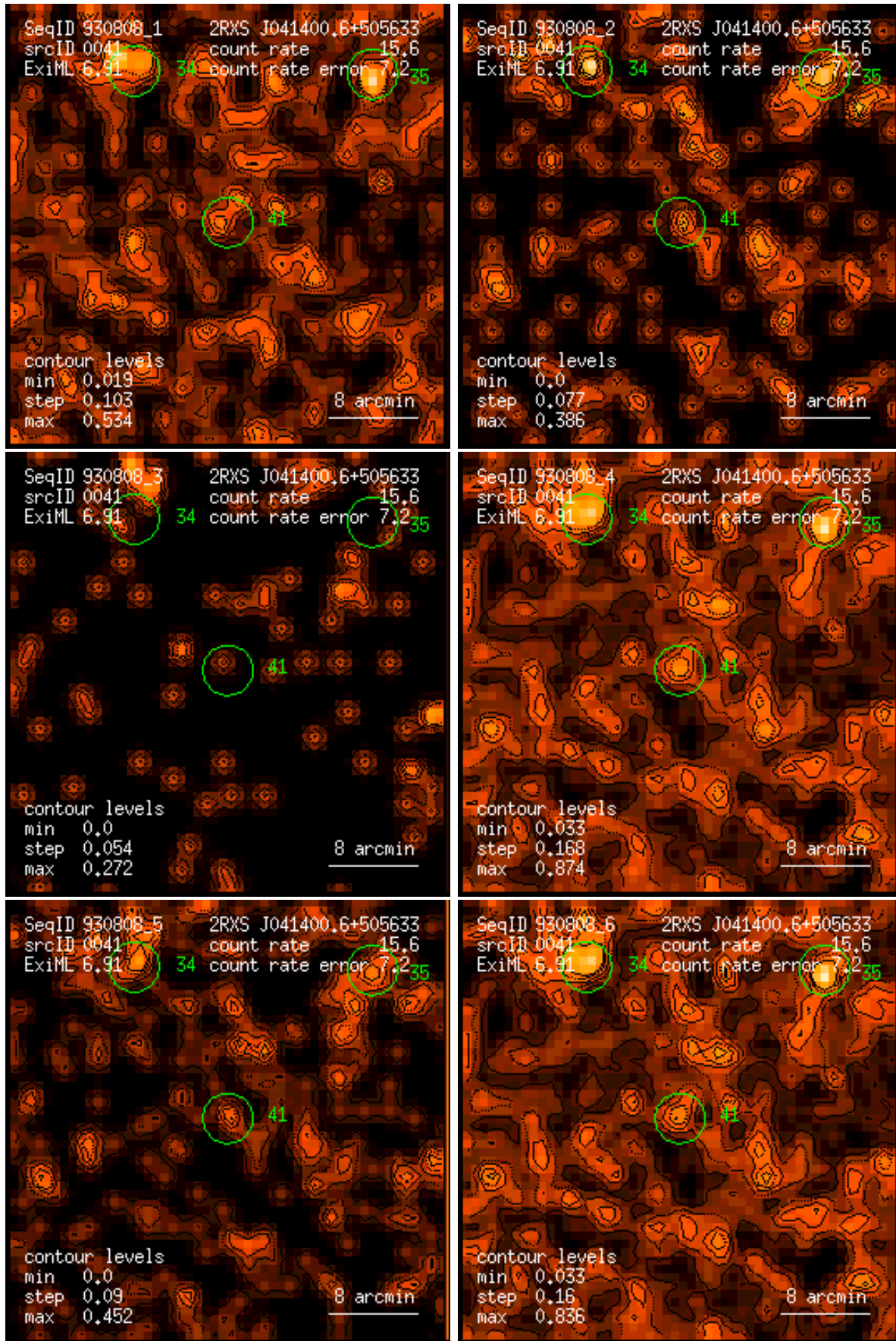
Figure 41: RASS 930808: detection 0041: band rate images, Gaussian filter: (1) PSPC channels 11 – 41, (2) 52 – 90, (3) 91 – 201, (4) 11 – 235, (5) 52 – 201, (6) 11 – 201. Broad band rates in counts/ks. Band rate contour levels in counts/ks/arcmin 2 .
