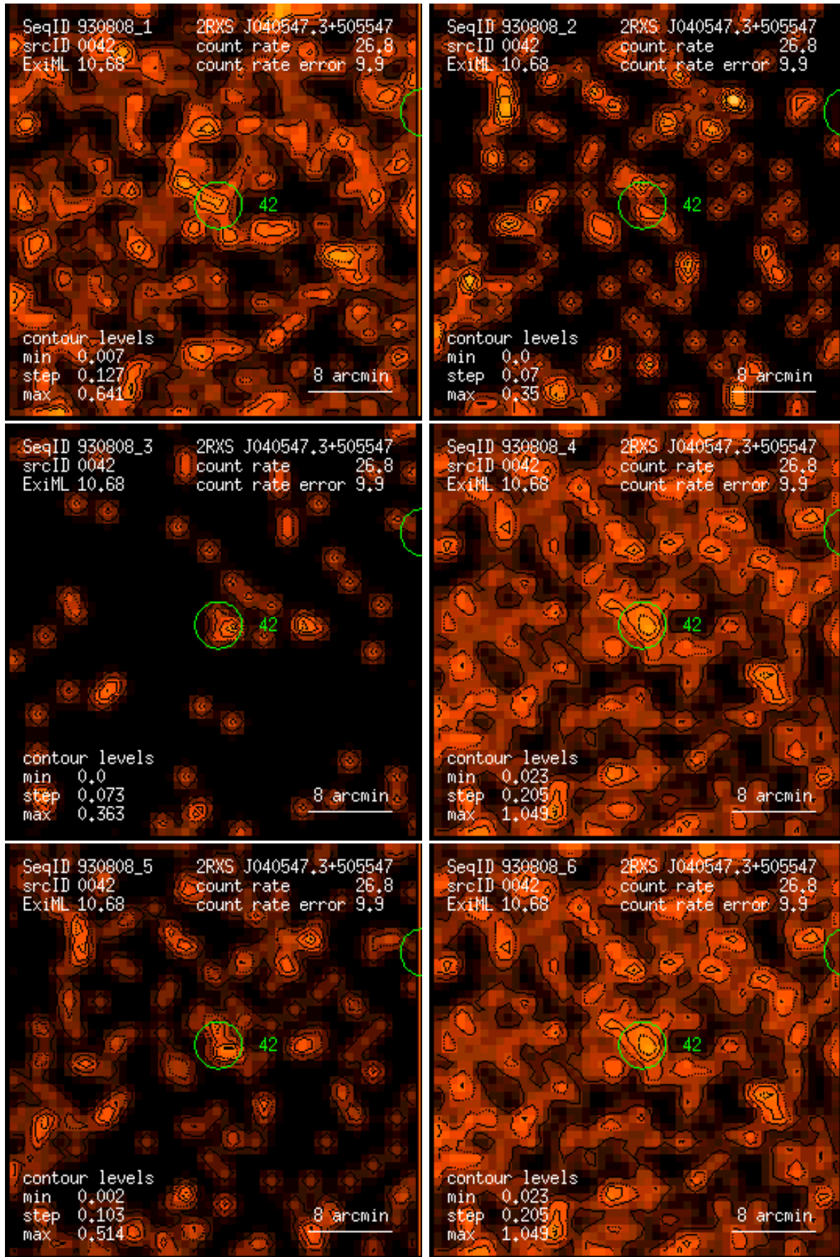
Figure 42: RASS 930808: detection 0042: band rate images, Gaussian filter: (1) PSPC channels 11 – 41, (2) 52 – 90, (3) 91 – 201, (4) 11 – 235, (5) 52 – 201, (6) 11 – 201. Broad band rates in counts/ks. Band rate contour levels in counts/ks/arcmin 2 .
