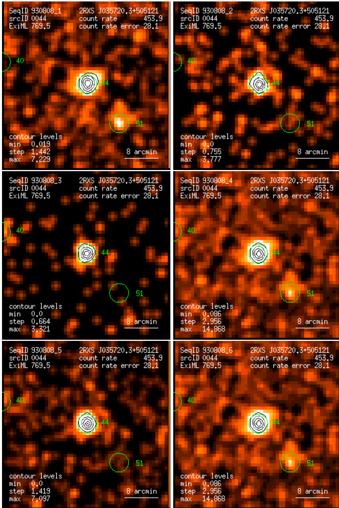
Figure 44: RASS 930808: detection 0044: band rate images, Gaussian filter: (1) PSPC channels 11 – 41, (2) 52 – 90, (3) 91 – 201, (4) 11 – 235, (5) 52 – 201, (6) 11 – 201. Broad band rates in counts/ks. Band rate contour levels in counts/ks/arcmin 2 .
