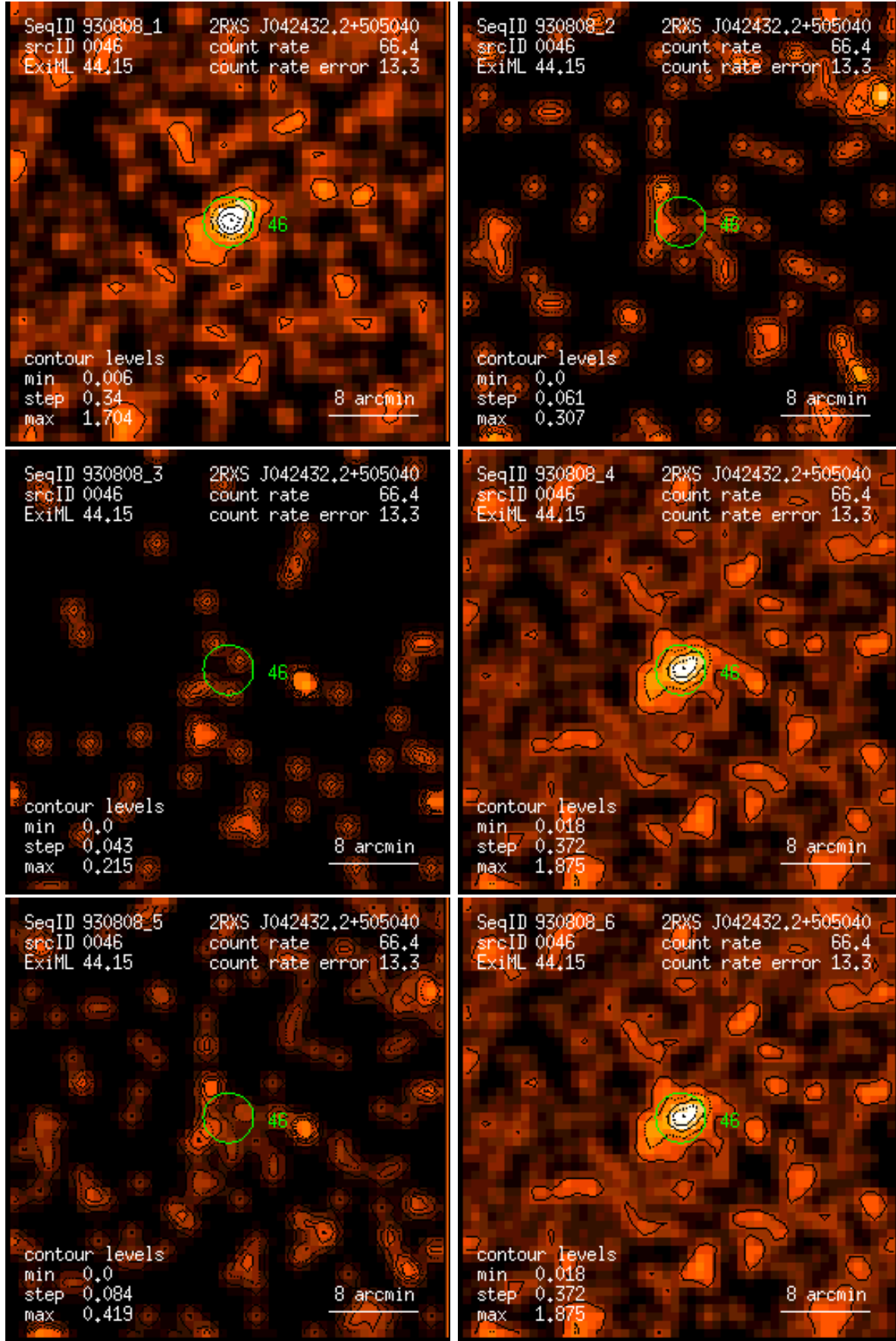
Figure 46: RASS 930808: detection 0046: band rate images, Gaussian filter: (1) PSPC channels 11 – 41, (2) 52 – 90, (3) 91 – 201, (4) 11 – 235, (5) 52 – 201, (6) 11 – 201. Broad band rates in counts/ks. Band rate contour levels in counts/ks/arcmin 2 .
