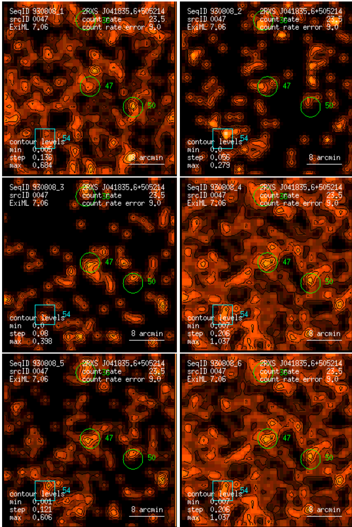
Figure 47: RASS 930808: detection 0047: band rate images, Gaussian filter: (1) PSPC channels 11 – 41, (2) 52 – 90, (3) 91 – 201, (4) 11 – 235, (5) 52 – 201, (6) 11 – 201. Broad band rates in counts/ks. Band rate contour levels in counts/ks/arcmin 2 .
