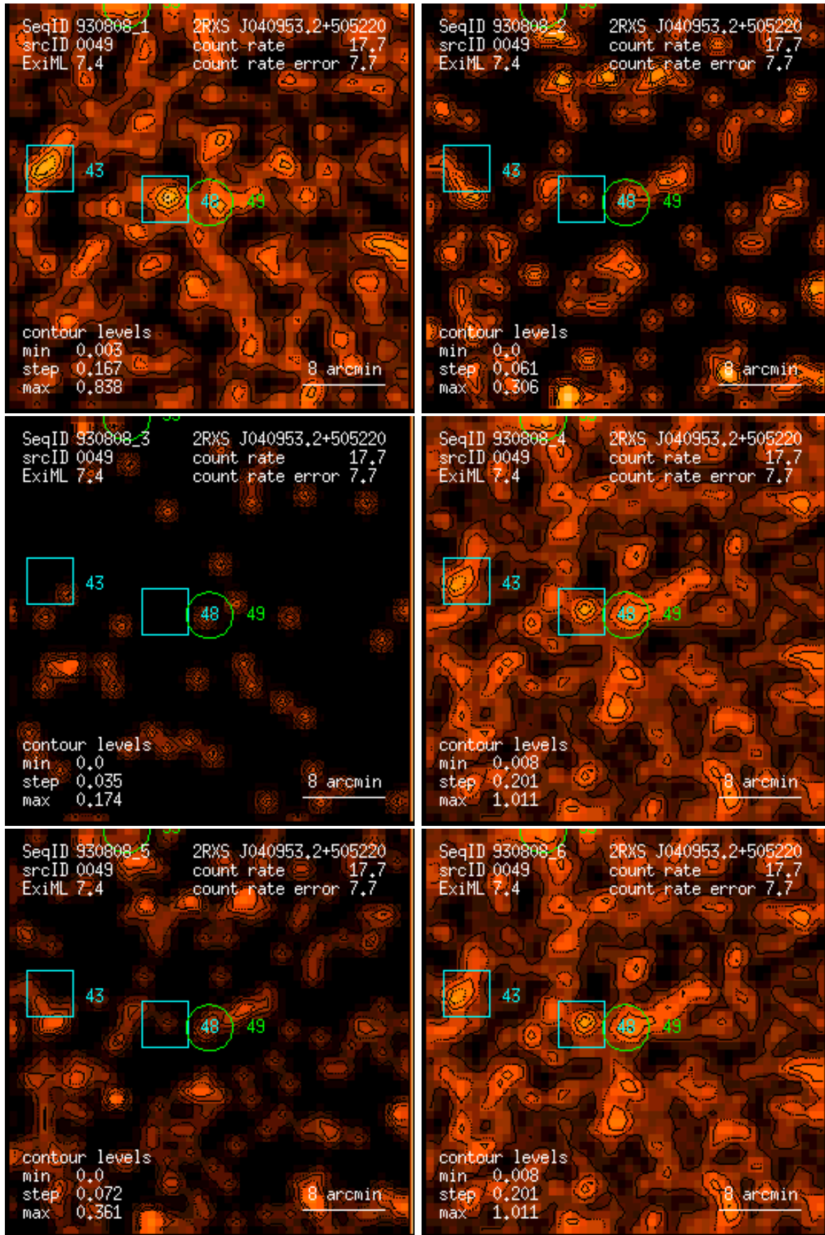
Figure 49: RASS 930808: detection 0049: band rate images, Gaussian filter: (1) PSPC channels 11 – 41, (2) 52 – 90, (3) 91 – 201, (4) 11 – 235, (5) 52 – 201, (6) 11 – 201. Broad band rates in counts/ks. Band rate contour levels in counts/ks/arcmin 2 .
