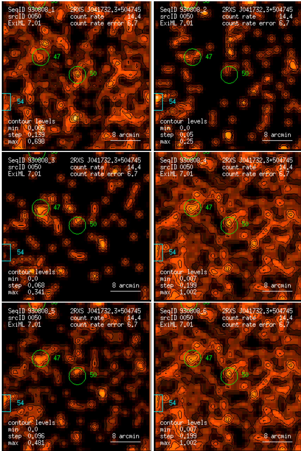
Figure 50: RASS 930808: detection 0050: band rate images, Gaussian filter: (1) PSPC channels 11 – 41, (2) 52 – 90, (3) 91 – 201, (4) 11 – 235, (5) 52 – 201, (6) 11 – 201. Broad band rates in counts/ks. Band rate contour levels in counts/ks/arcmin 2 .
