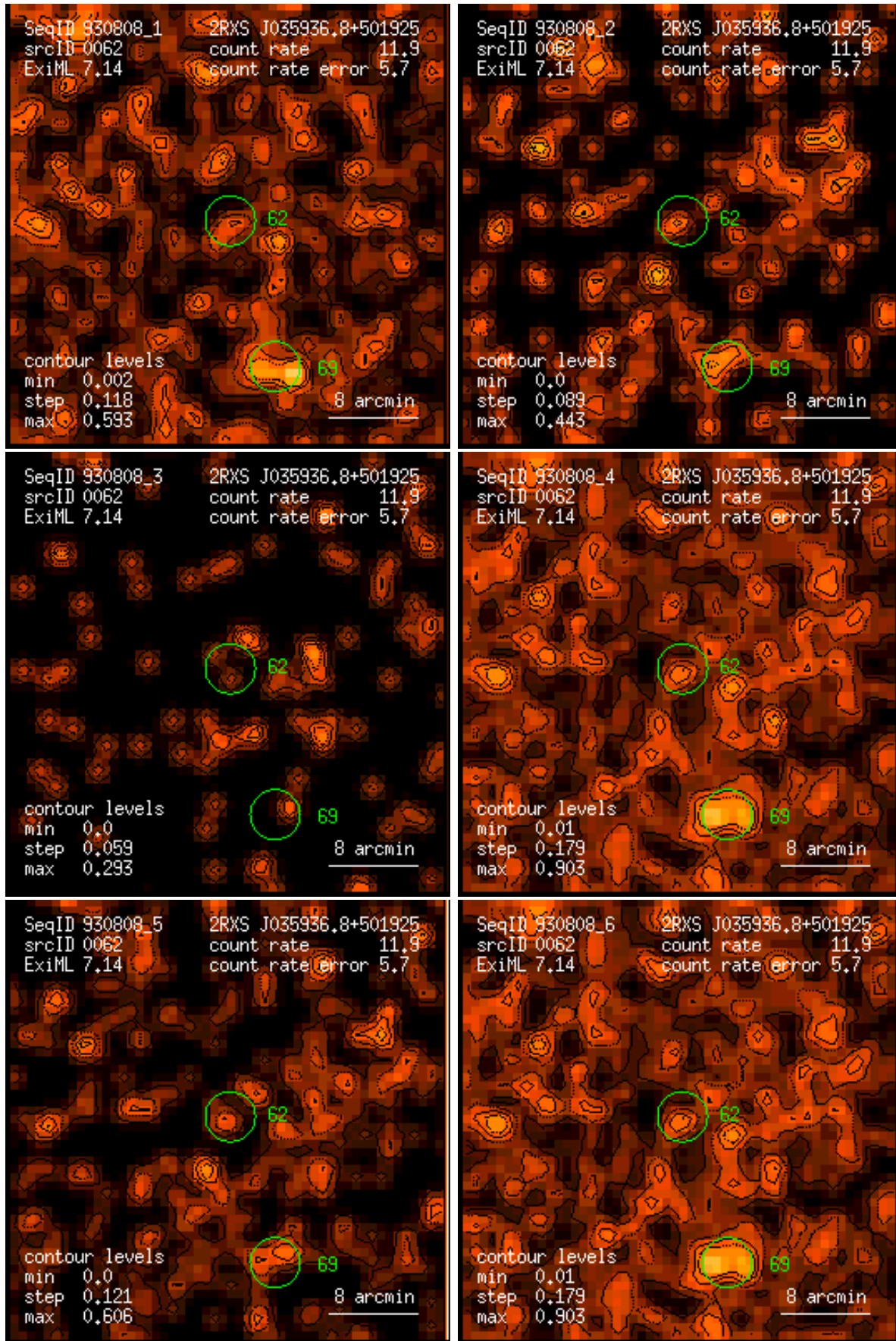
Figure 62: RASS 930808: detection 0062: band rate images, Gaussian filter: (1) PSPC channels 11 – 41, (2) 52 – 90, (3) 91 – 201, (4) 11 – 235, (5) 52 – 201, (6) 11 – 201. Broad band rates in counts/ks. Band rate contour levels in counts/ks/arcmin 2 .
