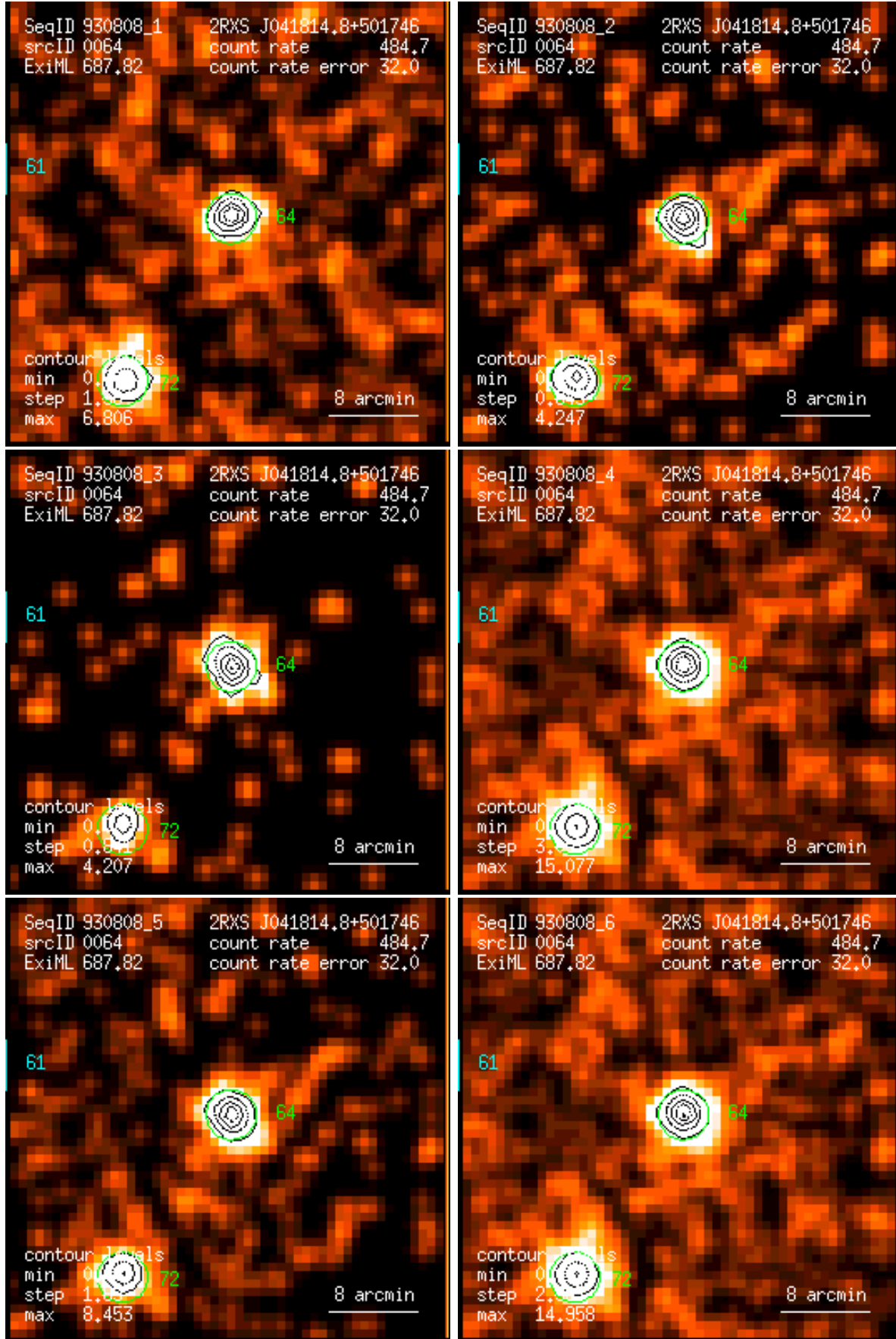
Figure 64: RASS 930808: detection 0064: band rate images, Gaussian filter: (1) PSPC channels 11 – 41, (2) 52 – 90, (3) 91 – 201, (4) 11 – 235, (5) 52 – 201, (6) 11 – 201. Broad band rates in counts/ks. Band rate contour levels in counts/ks/arcmin 2 .
