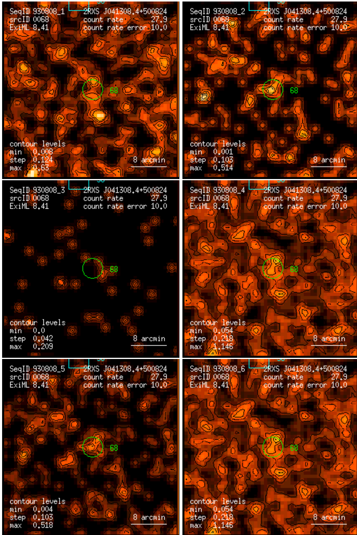
Figure 68: RASS 930808: detection 0068: band rate images, Gaussian filter: (1) PSPC channels 11 – 41, (2) 52 – 90, (3) 91 – 201, (4) 11 – 235, (5) 52 – 201, (6) 11 – 201. Broad band rates in counts/ks. Band rate contour levels in counts/ks/arcmin 2 .
