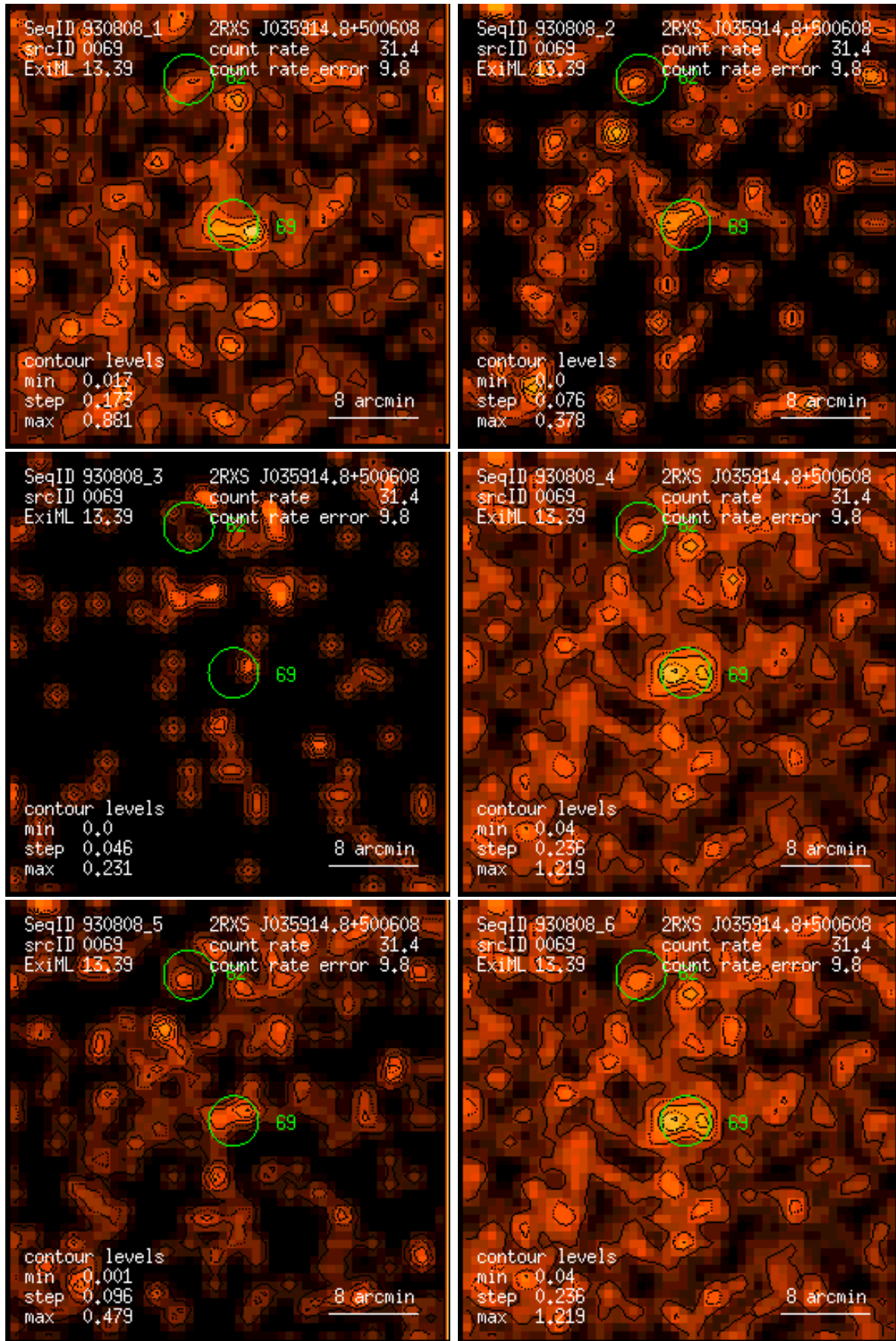
Figure 69: RASS 930808: detection 0069: band rate images, Gaussian filter: (1) PSPC channels 11 – 41, (2) 52 – 90, (3) 91 – 201, (4) 11 – 235, (5) 52 – 201, (6) 11 – 201. Broad band rates in counts/ks. Band rate contour levels in counts/ks/arcmin 2 .
