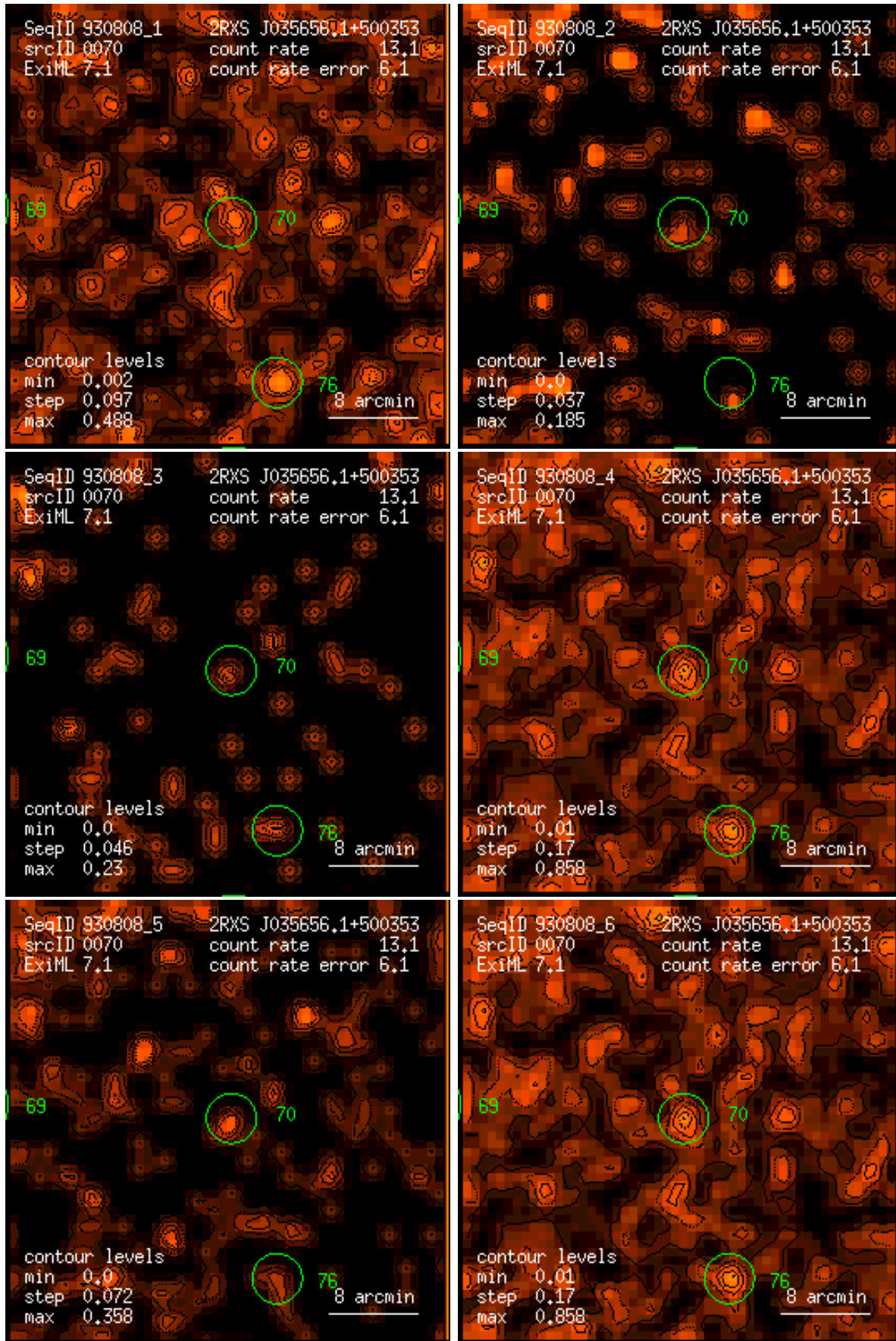
Figure 70: RASS 930808: detection 0070: band rate images, Gaussian filter: (1) PSPC channels 11 – 41, (2) 52 – 90, (3) 91 – 201, (4) 11 – 235, (5) 52 – 201, (6) 11 – 201. Broad band rates in counts/ks. Band rate contour levels in counts/ks/arcmin 2 .
