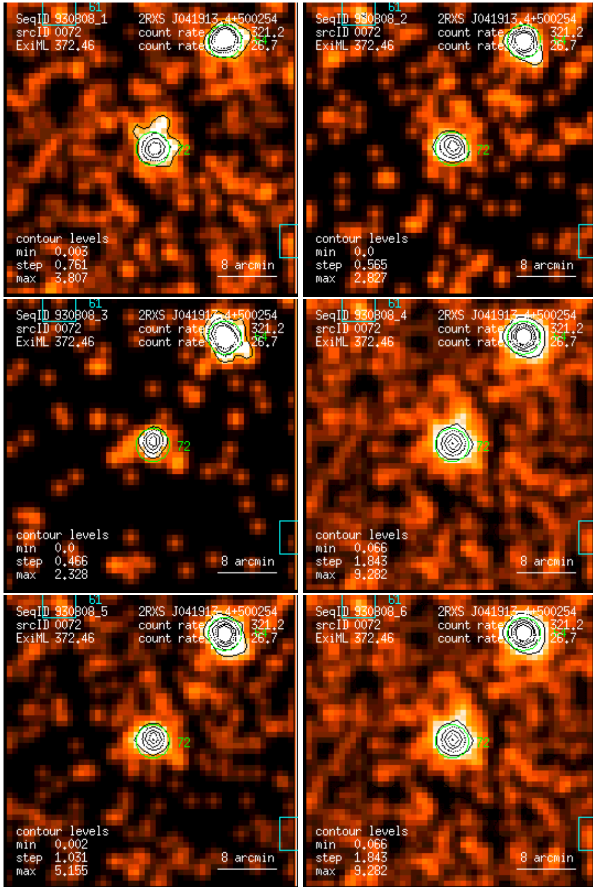
Figure 72: RASS 930808: detection 0072: band rate images, Gaussian filter: (1) PSPC channels 11 – 41, (2) 52 – 90, (3) 91 – 201, (4) 11 – 235, (5) 52 – 201, (6) 11 – 201. Broad band rates in counts/ks. Band rate contour levels in counts/ks/arcmin 2 .
