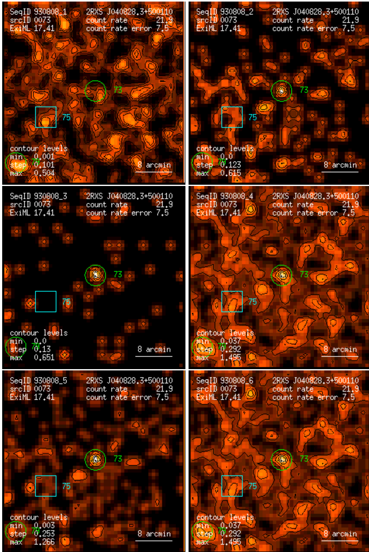
Figure 73: RASS 930808: detection 0073: band rate images, Gaussian filter: (1) PSPC channels 11 – 41, (2) 52 – 90, (3) 91 – 201, (4) 11 – 235, (5) 52 – 201, (6) 11 – 201. Broad band rates in counts/ks. Band rate contour levels in counts/ks/arcmin 2 .
