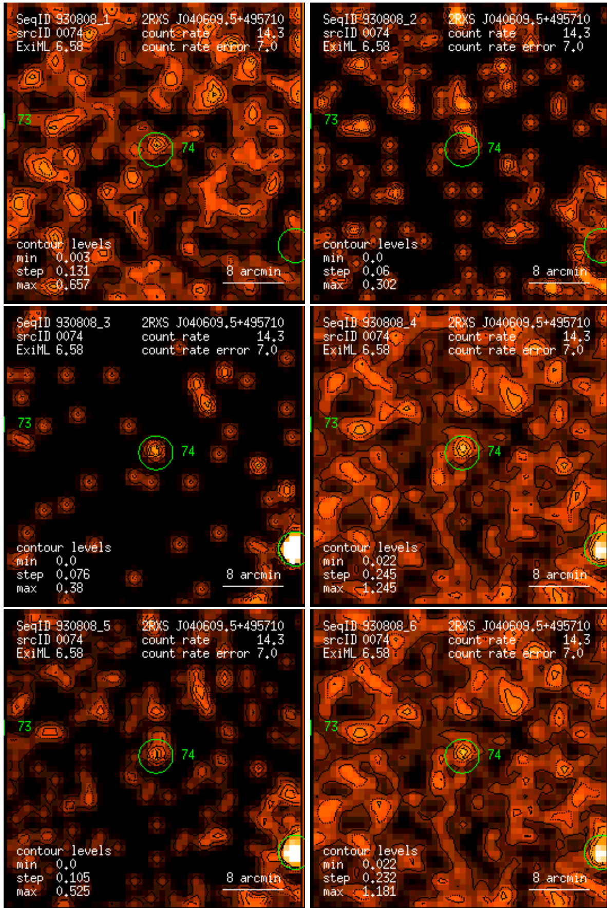
Figure 74: RASS 930808: detection 0074: band rate images, Gaussian filter: (1) PSPC channels 11 – 41, (2) 52 – 90, (3) 91 – 201, (4) 11 – 235, (5) 52 – 201, (6) 11 – 201. Broad band rates in counts/ks. Band rate contour levels in counts/ks/arcmin 2 .
