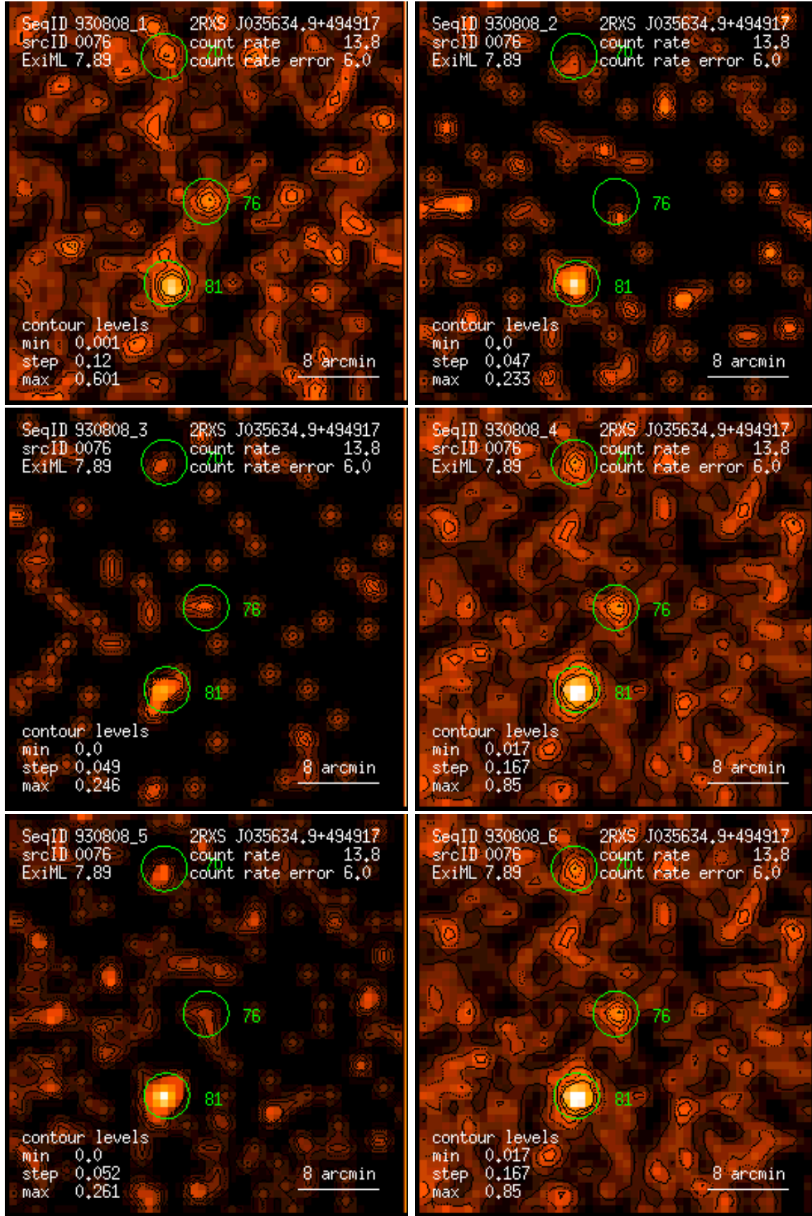
Figure 76: RASS 930808: detection 0076: band rate images, Gaussian filter: (1) PSPC channels 11 – 41, (2) 52 – 90, (3) 91 – 201, (4) 11 – 235, (5) 52 – 201, (6) 11 – 201. Broad band rates in counts/ks. Band rate contour levels in counts/ks/arcmin 2 .
