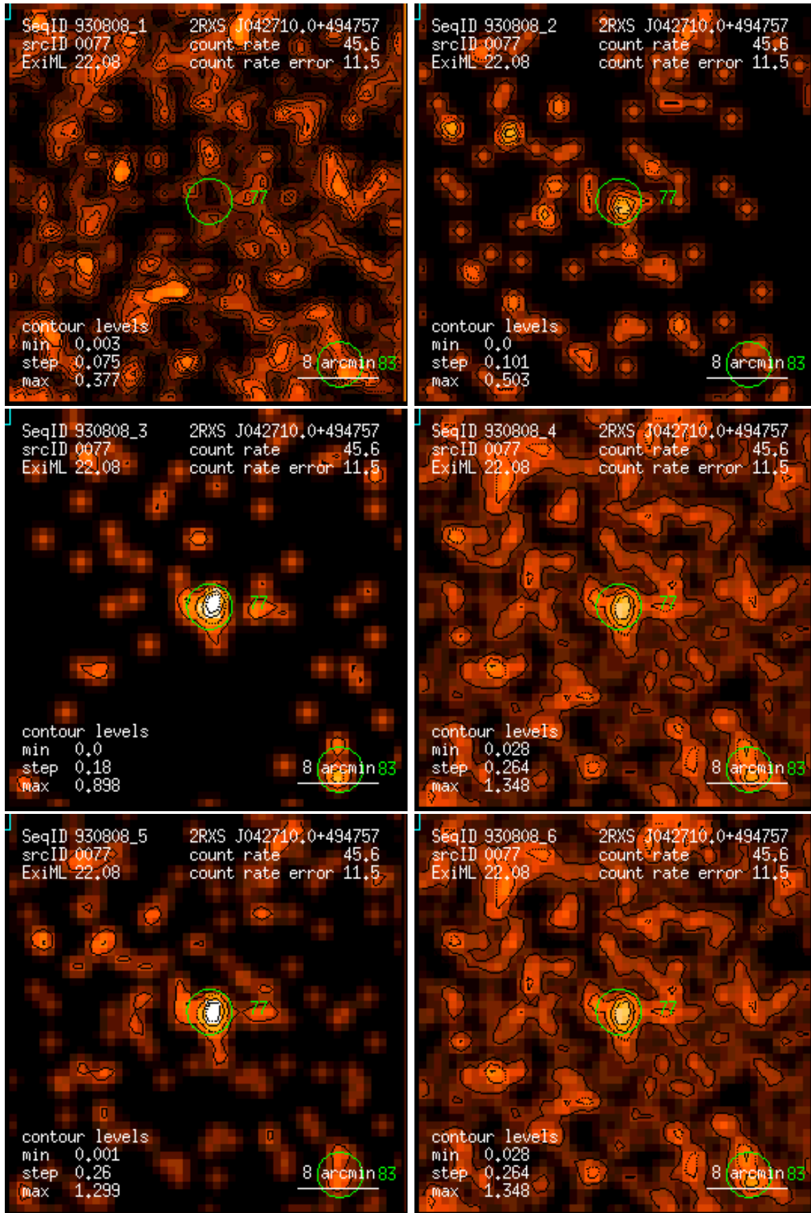
Figure 77: RASS 930808: detection 0077: band rate images, Gaussian filter: (1) PSPC channels 11 – 41, (2) 52 – 90, (3) 91 – 201, (4) 11 – 235, (5) 52 – 201, (6) 11 – 201. Broad band rates in counts/ks. Band rate contour levels in counts/ks/arcmin 2 .
