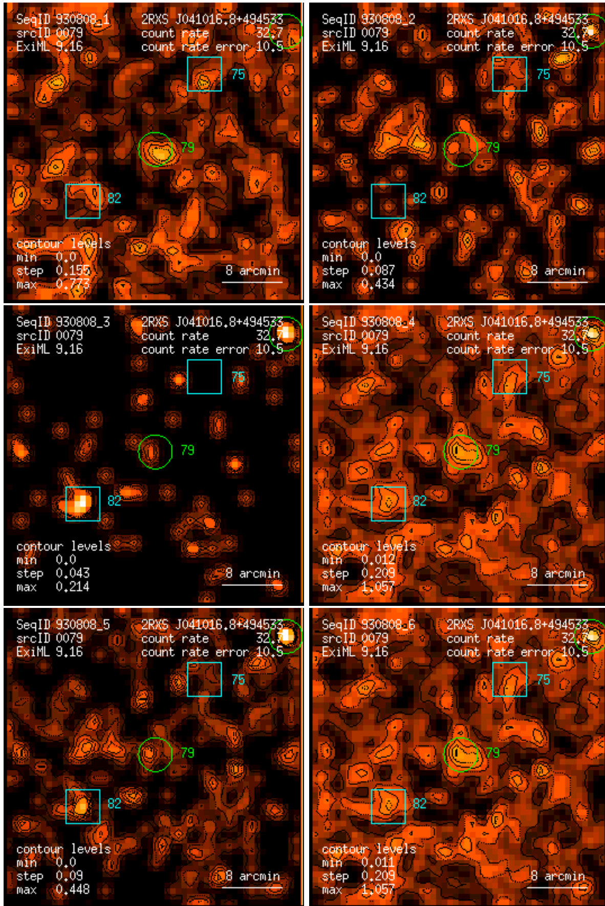
Figure 79: RASS 930808: detection 0079: band rate images, Gaussian filter: (1) PSPC channels 11 – 41, (2) 52 – 90, (3) 91 – 201, (4) 11 – 235, (5) 52 – 201, (6) 11 – 201. Broad band rates in counts/ks. Band rate contour levels in counts/ks/arcmin 2 .
