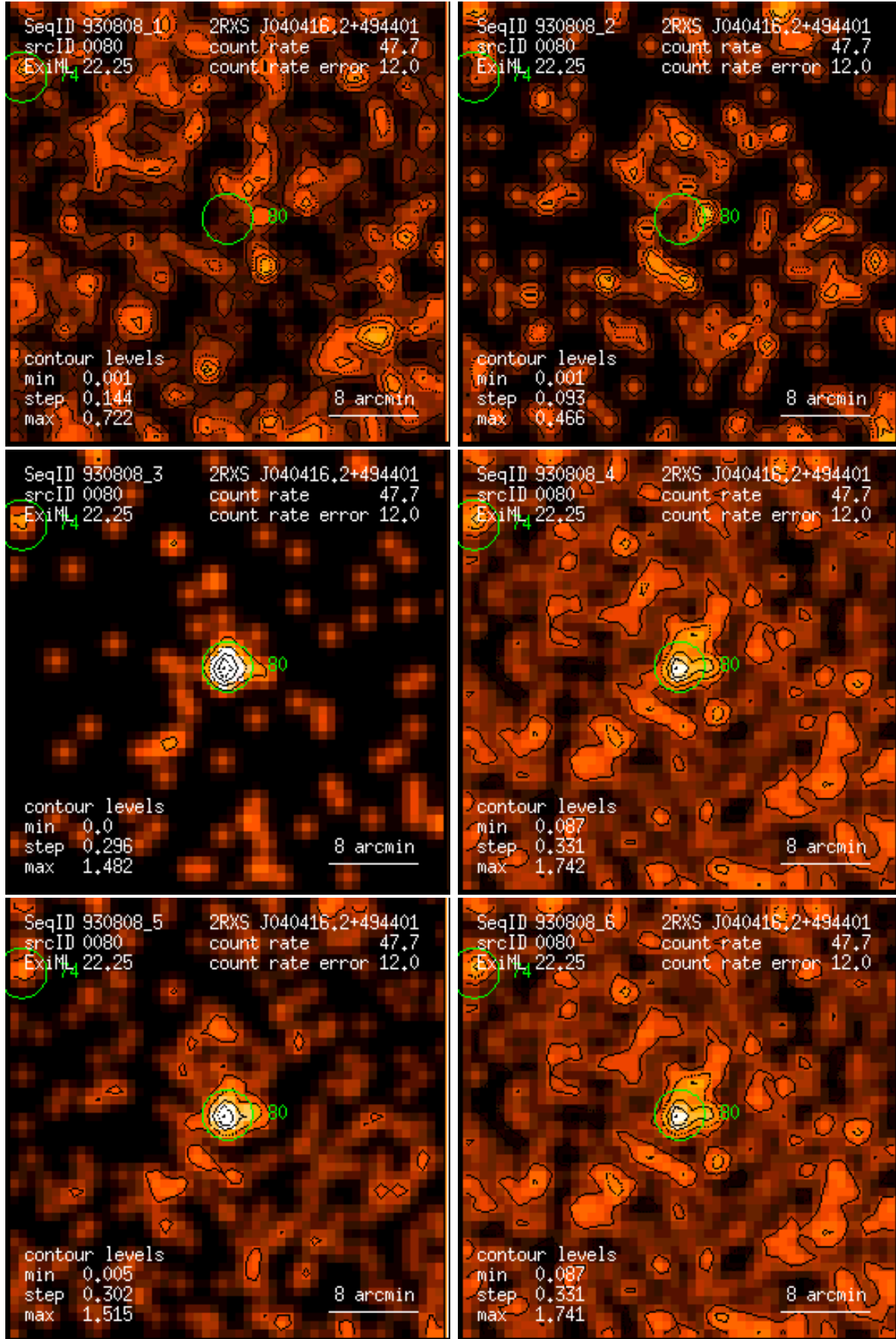
Figure 80: RASS 930808: detection 0080: band rate images, Gaussian filter: (1) PSPC channels 11 – 41, (2) 52 – 90, (3) 91 – 201, (4) 11 – 235, (5) 52 – 201, (6) 11 – 201. Broad band rates in counts/ks. Band rate contour levels in counts/ks/arcmin 2 .
