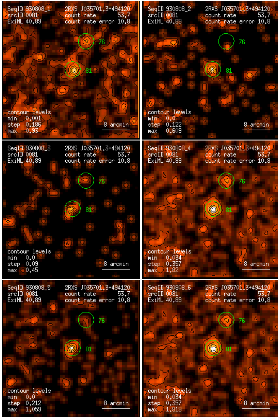
Figure 81: RASS 930808: detection 0081: band rate images, Gaussian filter: (1) PSPC channels 11 – 41, (2) 52 – 90, (3) 91 – 201, (4) 11 – 235, (5) 52 – 201, (6) 11 – 201. Broad band rates in counts/ks. Band rate contour levels in counts/ks/arcmin 2 .
