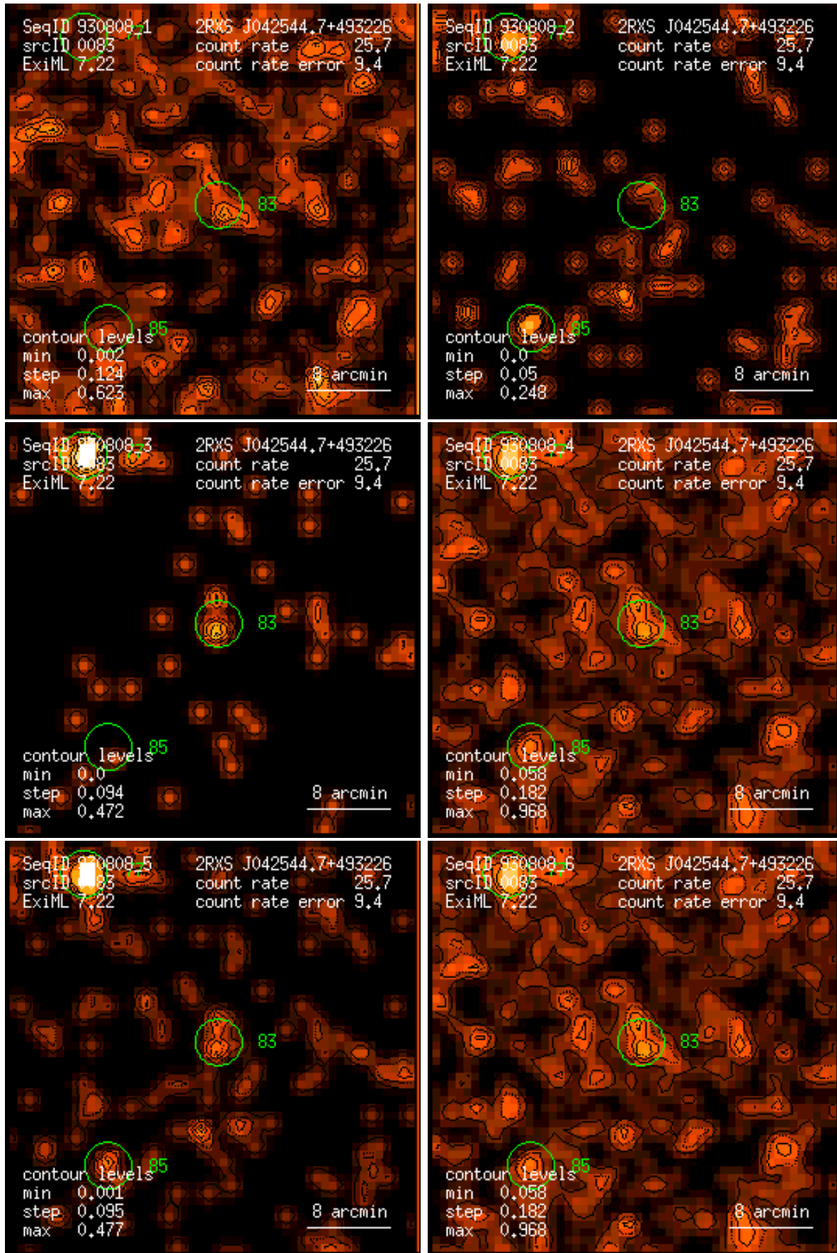
Figure 83: RASS 930808: detection 0083: band rate images, Gaussian filter: (1) PSPC channels 11 – 41, (2) 52 – 90, (3) 91 – 201, (4) 11 – 235, (5) 52 – 201, (6) 11 – 201. Broad band rates in counts/ks. Band rate contour levels in counts/ks/arcmin 2 .
