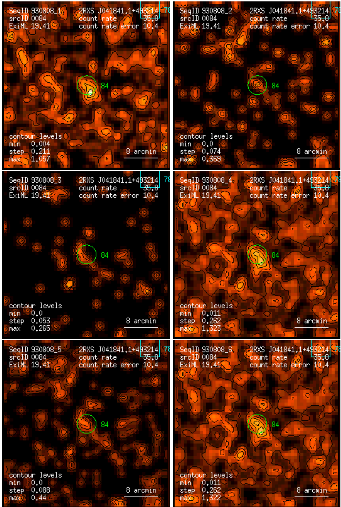
Figure 84: RASS 930808: detection 0084: band rate images, Gaussian filter: (1) PSPC channels 11 – 41, (2) 52 – 90, (3) 91 – 201, (4) 11 – 235, (5) 52 – 201, (6) 11 – 201. Broad band rates in counts/ks. Band rate contour levels in counts/ks/arcmin 2 .
