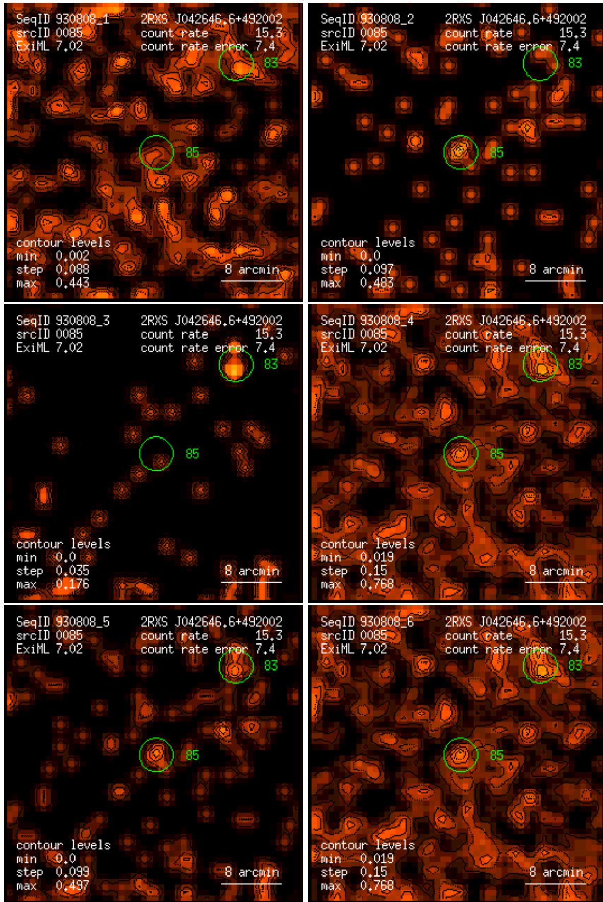
Figure 85: RASS 930808: detection 0085: band rate images, Gaussian filter: (1) PSPC channels 11 – 41, (2) 52 – 90, (3) 91 – 201, (4) 11 – 235, (5) 52 – 201, (6) 11 – 201. Broad band rates in counts/ks. Band rate contour levels in counts/ks/arcmin 2 .
