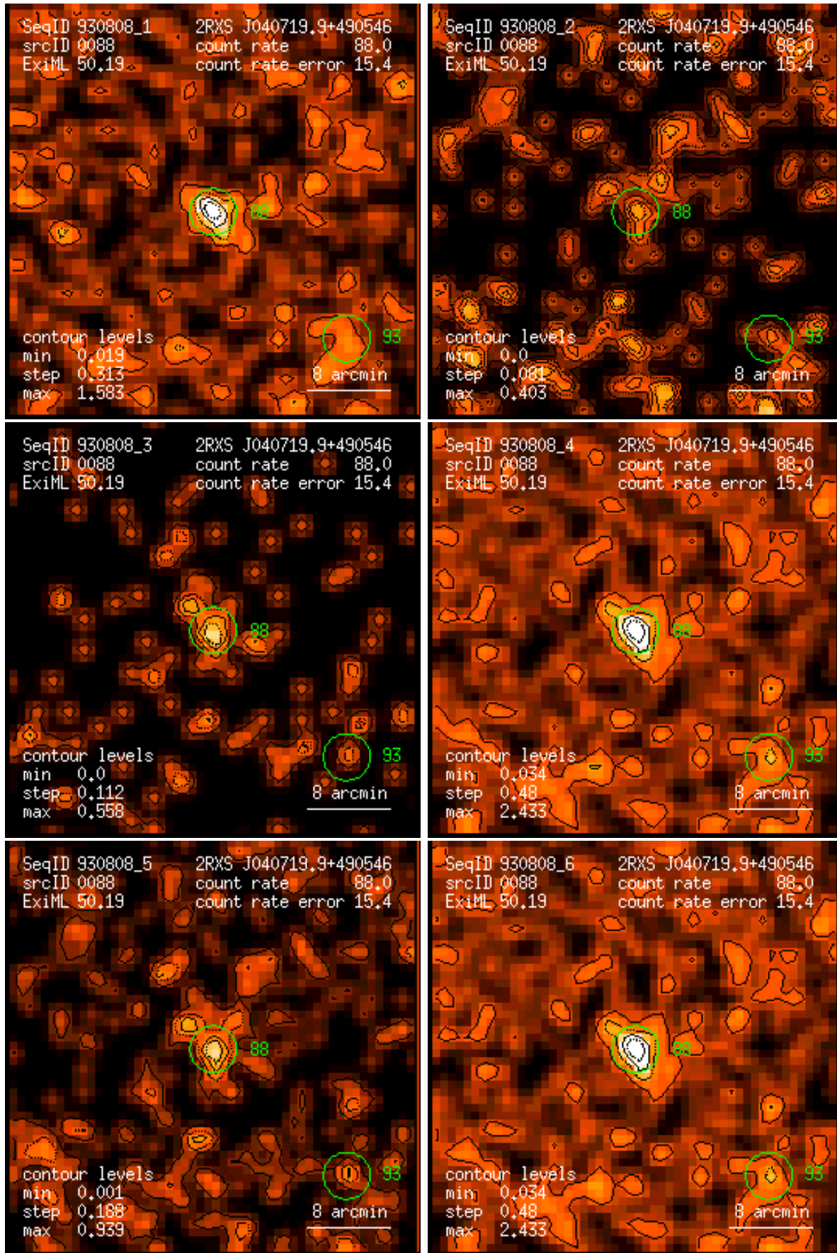
Figure 88: RASS 930808: detection 0088: band rate images, Gaussian filter: (1) PSPC channels 11 – 41, (2) 52 – 90, (3) 91 – 201, (4) 11 – 235, (5) 52 – 201, (6) 11 – 201. Broad band rates in counts/ks. Band rate contour levels in counts/ks/arcmin 2 .
