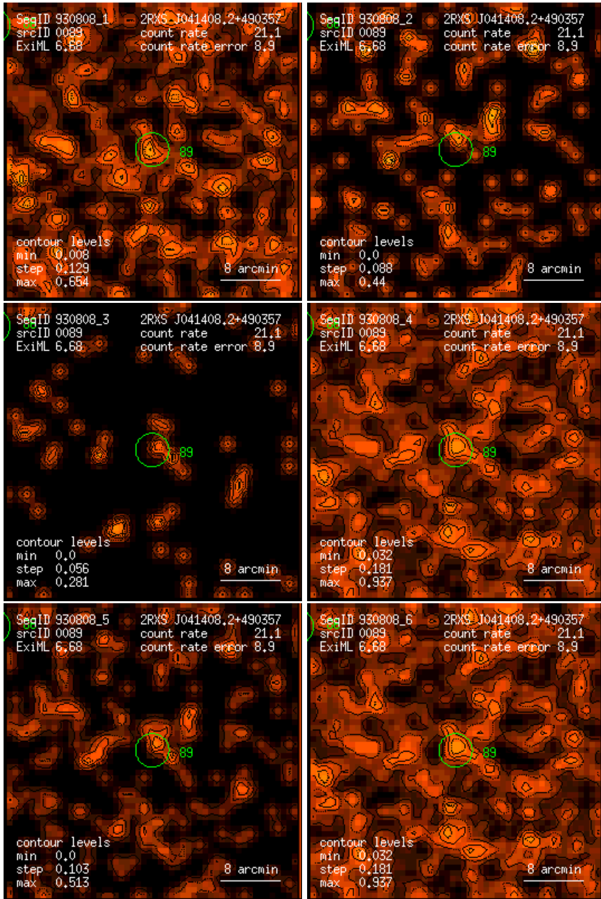
Figure 89: RASS 930808: detection 0089: band rate images, Gaussian filter: (1) PSPC channels 11 – 41, (2) 52 – 90, (3) 91 – 201, (4) 11 – 235, (5) 52 – 201, (6) 11 – 201. Broad band rates in counts/ks. Band rate contour levels in counts/ks/arcmin 2 .
