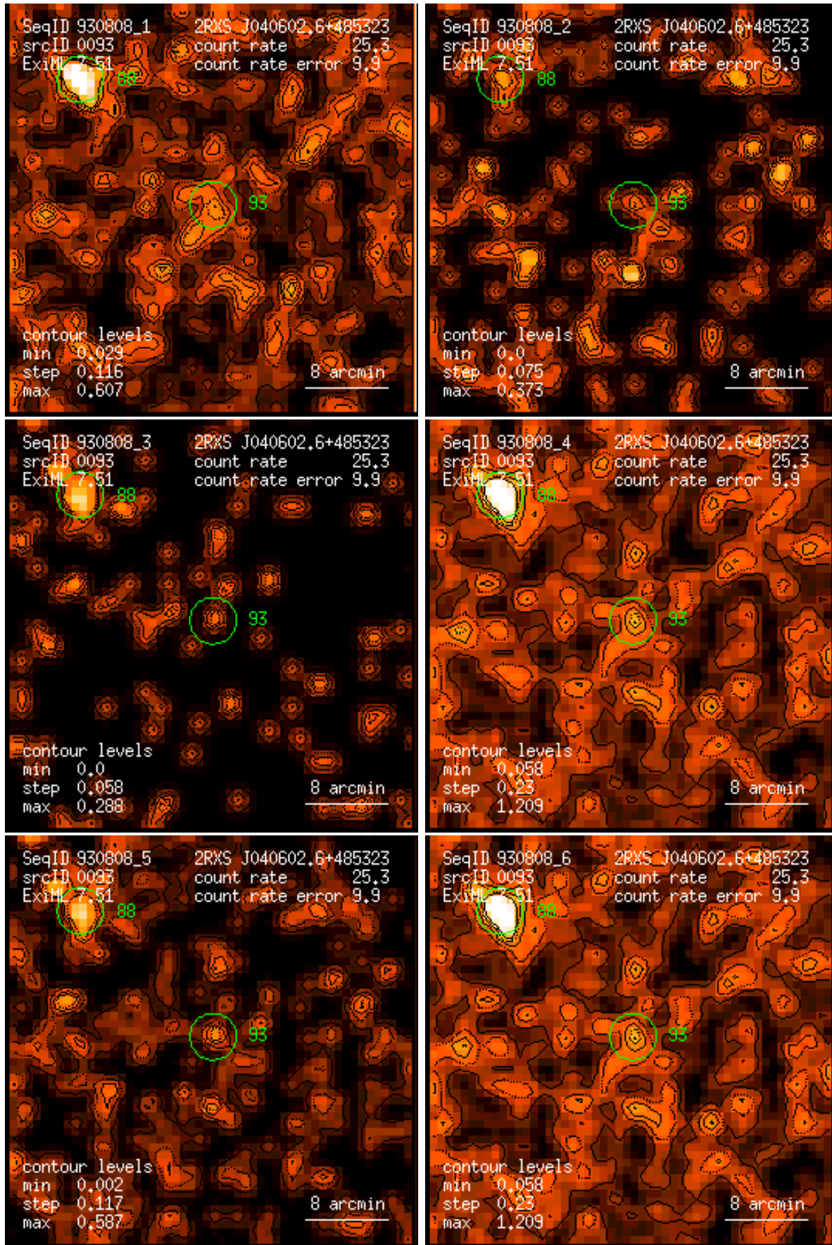
Figure 93: RASS 930808: detection 0093: band rate images, Gaussian filter: (1) PSPC channels 11 – 41, (2) 52 – 90, (3) 91 – 201, (4) 11 – 235, (5) 52 – 201, (6) 11 – 201. Broad band rates in counts/ks. Band rate contour levels in counts/ks/arcmin 2 .
