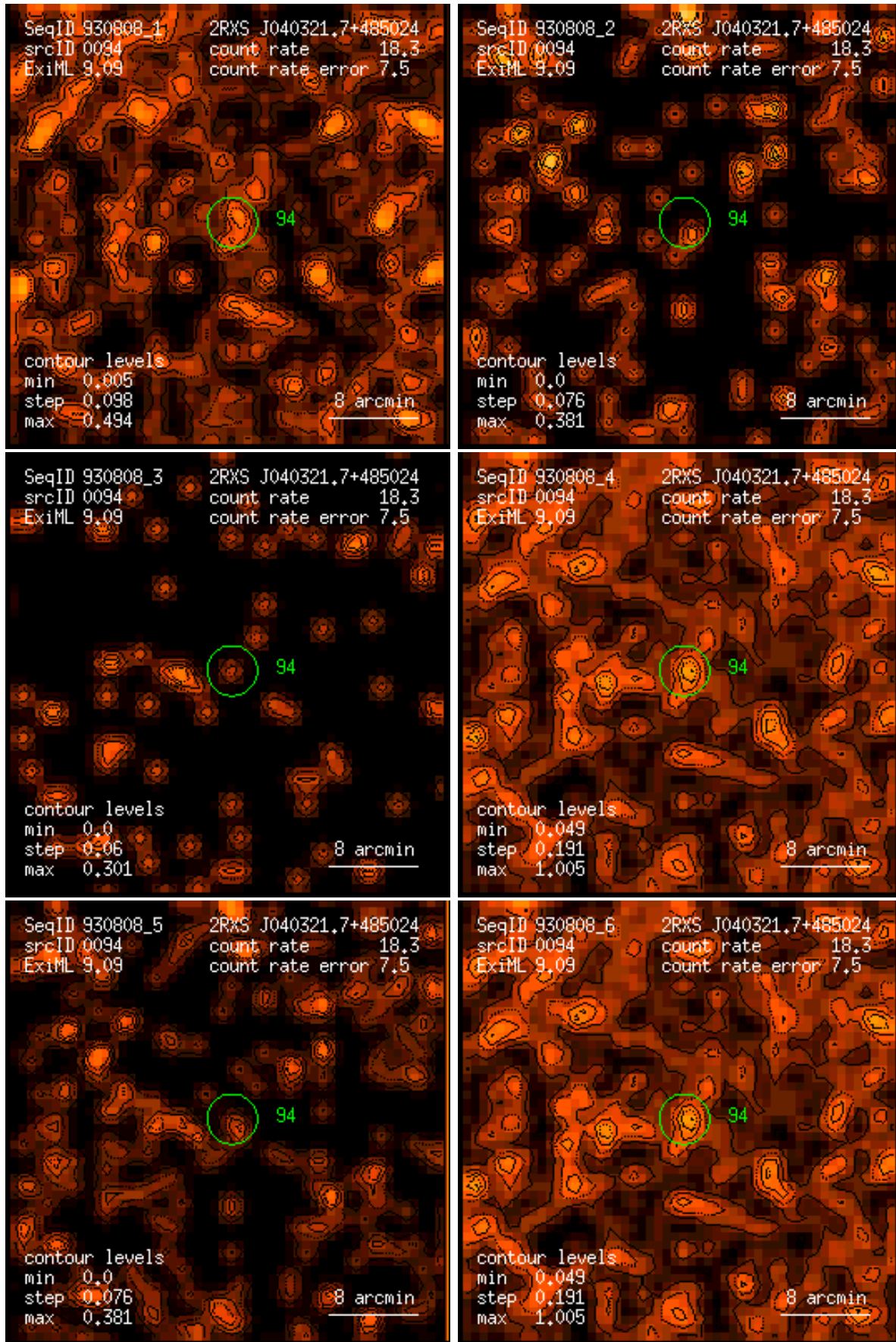
Figure 94: RASS 930808: detection 0094: band rate images, Gaussian filter: (1) PSPC channels 11 – 41, (2) 52 – 90, (3) 91 – 201, (4) 11 – 235, (5) 52 – 201, (6) 11 – 201. Broad band rates in counts/ks. Band rate contour levels in counts/ks/arcmin 2 .
